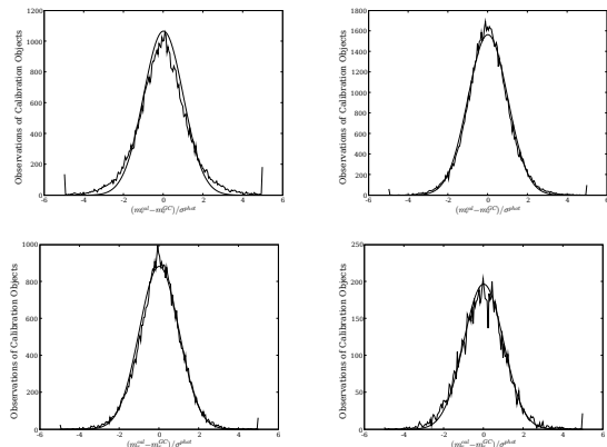
Figure 15. Distributions of “pulls” of the calibration second-order model fit for observations with photometric error \sigma^{phot} in ranges, (top left) 0.00 - 0.01, (top right) 0.01 - 0.02, (bottom left) 0.02 - 0.04, and (bottom right) 0.04 - 0.10. Overflow and underflow counts are shown at \pm 5 on the horizontal axis. Overlaid on the data are Gaussian distributions with s.d. = 1.0 and normalized to the total number of observations.
