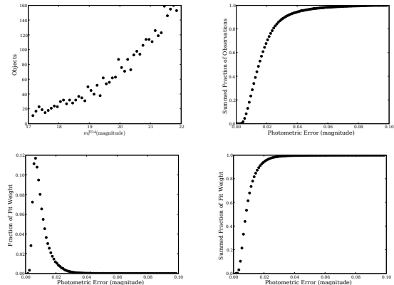
Figure 14. Distribution (top left) of magnitudes of calibration objects; cumulative distribution (top right) of photometric errors of observations of calibration objects; distribution (bottom left) of weights in the global calibration fit; and cumulative distribution (bottom right) of calibration weights.
