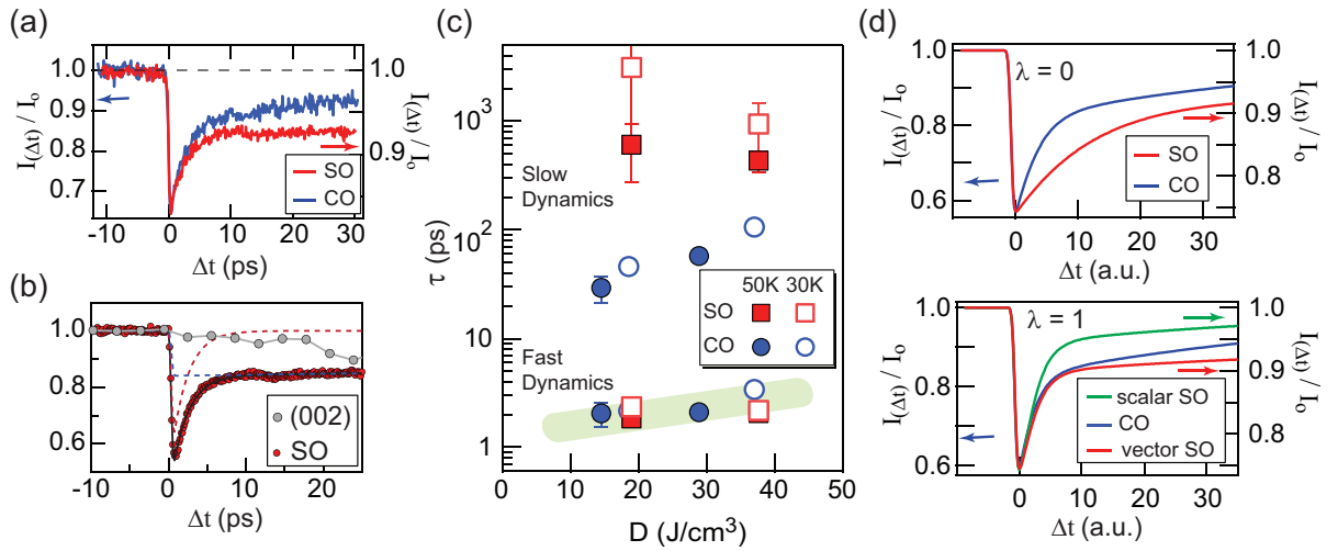
FIG. 3: (color online) (a) Time traces of the normalized CO (blue curve, left axis) and SO (red curve, right axis) peak intensities at a photo-excitation density of approximately 19 J/cm^3 at 30 K. (b) Two-time-scale model fitting (black curve) to the SO time trace (red curve). The fitted initial fast (red dashed curve) and slow (blue dashed curve) dynamics are also plotted. The data of (0,0,2) Bragg peak are also included to illustrate a very different lattice dynamics than those exhibited in CO and SO. The demonstrated SO and (0,0,2) Bragg peak data were taken at 50 K with an excitation densities of 38 J/cm^3 . (c) A summary plot of the fast and slow time scales of the CO[27] (blue circles) and SO (red squares) as a function of photo-excitation density. The green shaded area is a guide-to-the-eye to highlight a comparable fast time scale for the CO and SO. The dynamics at 30 K (open markers) and 50 K (filled markers) are essentially the same within the experimental uncertainties. The error bars are determined by 95% confidence interval of fitting. The long-lived meta-stable state of SO dynamics has a life time much longer than the recorded time window, yielding a large error bar. (d) Simulated time traces of the normalized CO and SO peak intensities from time-dependent Ginzburg-Landau theory. The upper (lower) panel shows the results when the SO-CO coupling is zero (of the order 1). In the lower panel, the trace labeled with “vector SO” includes the SO vector re-orientation effect.
