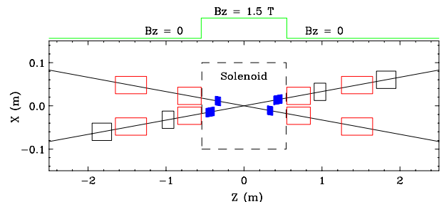
Figure 2: Effective hard-edge detector solenoid near IP.
