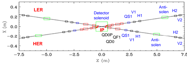
Figure 6: Solenoid correctors within \pm 7.5 m of IP.
