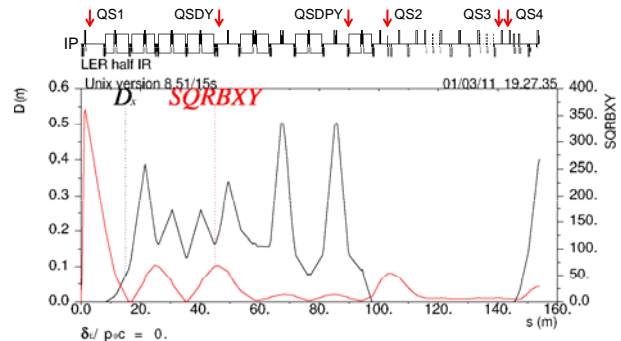
Figure 4: LER skew quadrupoles in half-IR. Plotted functions are dispersion and \sqrt{\beta_x \beta_y} .
