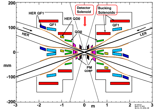
Figure 1: IR layout with detector and bucking solenoids.
