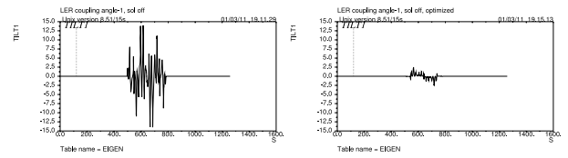
Figure 8: LER beam tilt angle (deg) for mode 1 with solenoid off. Left - original QDOP rotation, right - optimal QDOP rotation.
