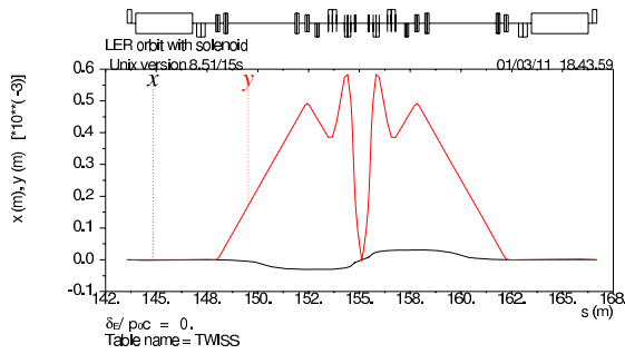
Figure 5: Corrected orbit in the LER IR.
