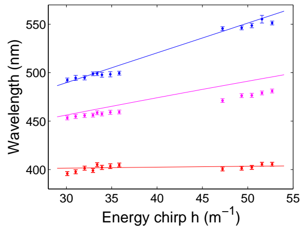
Figure 6: Radiation wavelength vs beam energy chirp for the echo signal E2 (red), E3 (magenta) and that from the 795 nm laser alone H2 (blue). Straight lines are prediction from HGHG and EEHG theory (Eq. 1).
