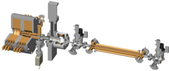
Figure 1. The low energy portion of the LLNL and SLAC photoinjectors include a 5.6-cell X-band RF Gun and a T53 or T105 structure.
