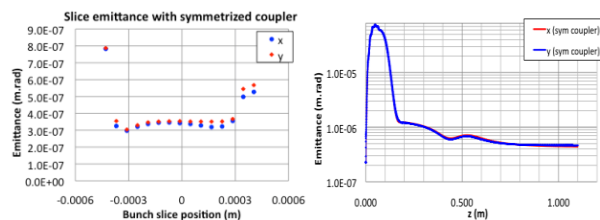
Figure 7. Slice and projected emittances with symmetrized couplers at the end of the first accelerator.
