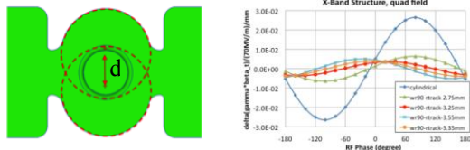
Figure 5. Left: Racetrack cell shape for quadrupole compensation. Right: quad strength with/without compensation for the T53 coupler at 70 MV gradient.
