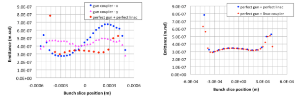
Figure 3. Top: Head-tail emittance growth due to quad effects in the gun (left) and first accelerator (right).
