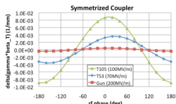
Figure 6. Residual phase related quadrupole fields after racetrack compensation.
