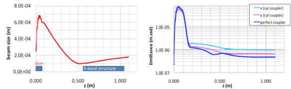
Figure 4. Transverse beam size and the projected emittance along the injector.
