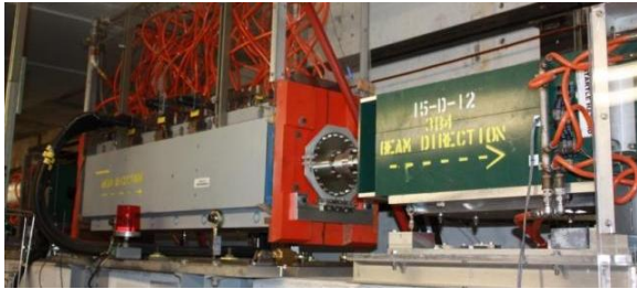
Figure 6: Energy spectrometer wiggler (left) and one chicane dipole (right) installed in ESA [6,7].
