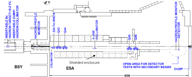
Figure 4: Layout of the hadron beam line diverging at 1.35^\circ from the un-deflected beam trajectory.
