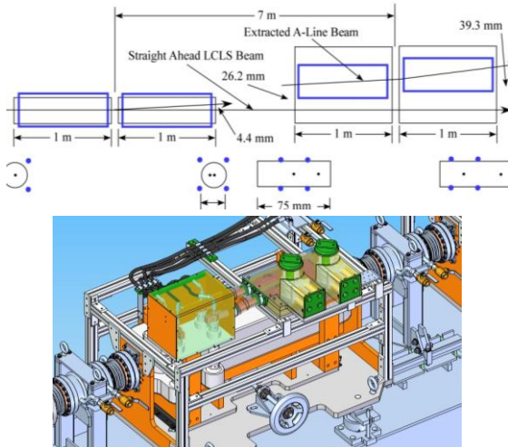
Figure 2: (above) Layout of the 4 kicker magnet system to kick the beam into ESA; (below) magnet assembly.
