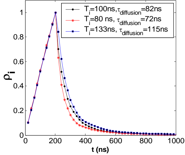
FIG. 9. Build-up of ion-cloud along a short bunch train and its decay during the train gap for various ions' oscillation frequencies. The ion density is normalized so that the peak density at the end of the bunch train is 1. The calculated ion oscillation period T_i and the simulated ion decay time \tau_{diffusion} during the bunch train gap are also shown in the plot.
