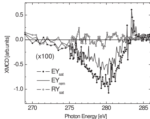
Figure 4. XMCD spectra ( \times 100 ) of the irradiated HOPG samples obtained using EY in an applied field of \pm 0.7 T ( \bullet ) or in remanence after saturating the sample in a field of \pm 0.7 T ( - ). Also shown is the XMCD spectrum acquired in saturation using the reflection yield ( \circ ). Lines are added as a guide to the eye. All spectra were obtained at \alpha = 45^\circ .
