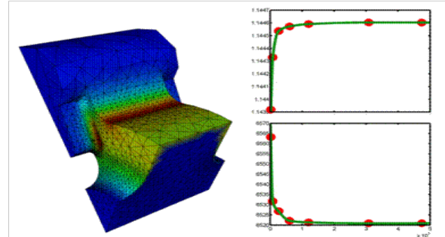
Figure 5. (Left) Field distribution of a cavity mode in the final mesh after adaptive refinement. (Right) Convergence of frequency (top) and Q (bottom) at different levels of mesh refinement.
