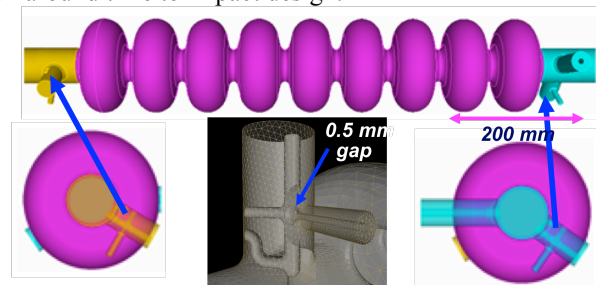
Figure 1. The ILC SRF cavity.
