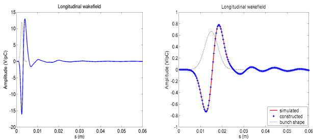
Figure 13. (Left) Short-range wakefield for the PEP-X undulator with a RMS bunch length 0.5 \mu\text{m} . (Right) Comparison of wakefield for 3 mm bunch with that reconstructed from 0.5 \mu\text{m} .
