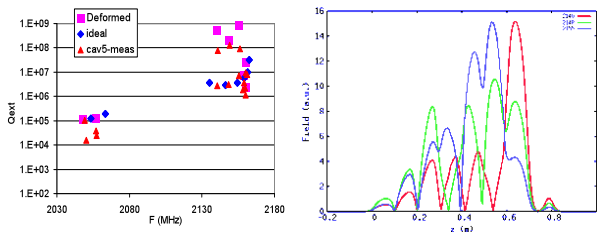
Figure 16. (Left) Q s of dipole modes for the calculated ideal cavity, deformed cavity and measurement; (Right) Field distributions of the high Q dipole modes shifted away from the HOM couplers and reduced damping.
