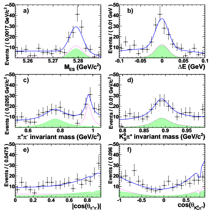
FIG. 1: Projections of the multidimensional fit onto (a) m_{ES} , (b) \Delta E , (c) \pi^+ \pi^- mass, (d) K_S^0 \pi^+ mass, (e) |\cos \theta_{\pi^+ \pi^-}| , and (f) \cos \theta_{K_S^0 \pi^+} for modes with K^{*+} \rightarrow K_S^0 \pi^+ . The points with error bars show the data; the solid line shows signal-plus-background; the green hatched area is the \rho^0 K^{*+} signal; and the red dashed line is the f_0(980) K^{*+} signal.
