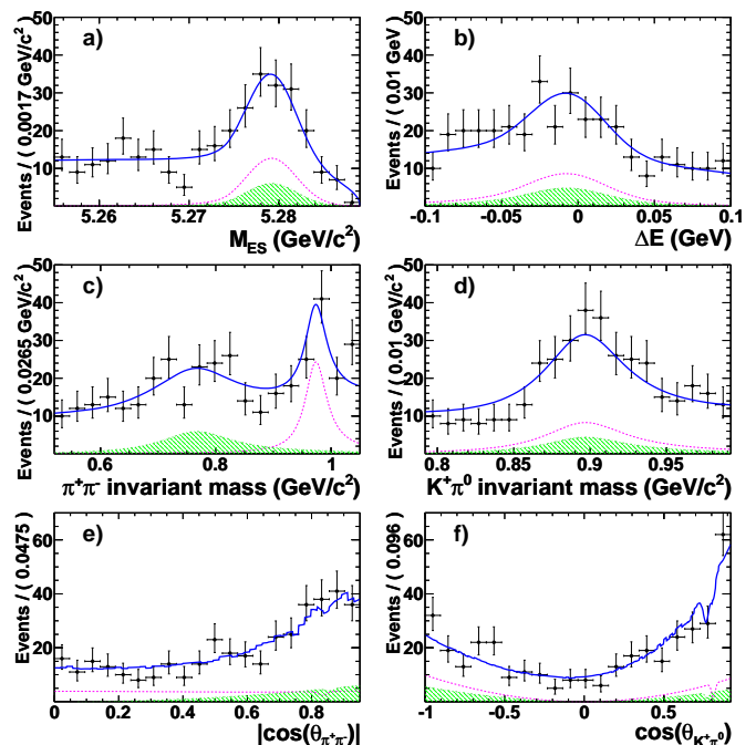
FIG. 2: Projections of the multidimensional fit onto (a) m_{ES} , (b) \Delta E , (c) \pi^+ \pi^- mass, (d) K^+ \pi^0 mass, (e) |\cos \theta_{\pi^+ \pi^-}| , and (f) \cos \theta_{K^+ \pi^0} for modes with K^{*+} \rightarrow K^+ \pi^0 . The same projection criteria and legend are used as in Fig. 1.
