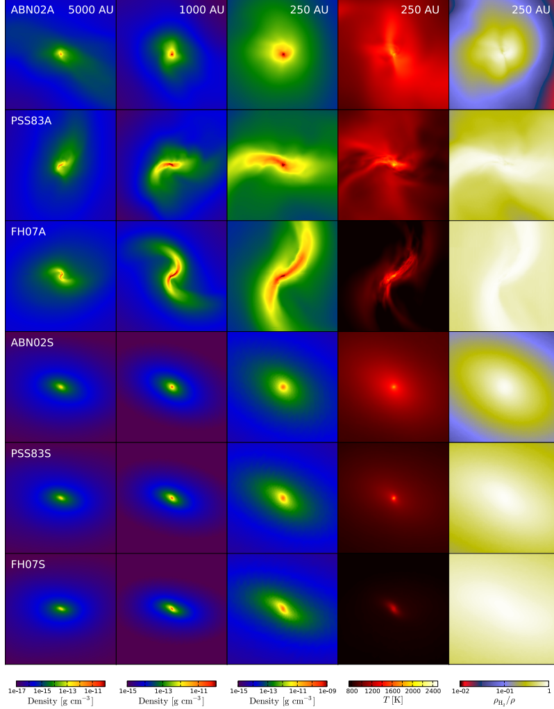
Fig. 6.— Mass-weighted average quantities, calculated along rays at every pixel. Rays are cast parallel to the angular momentum vector of the region in question for every column for the AMR simulations, and parallel to the Z axis for the SPH simulations. Rows correspond to simulations ABN02A, PSS83A, FH07A, ABN02S, PS83S and FH07S, and displayed values are calculated dividing mass-weighted accumulated values by the total column density at each ray. Column 1 shows density with a field of view and depth of ray integration of 5000 AU, column 2 shows density with a field of view and depth of integration of 1000 AU, and columns 3-5 show density, temperature and \text{H}_2 fraction with fields of view and depths of integration of 250 AU. These images were made from snapshots of the simulations at the time when their maximum density was 10^{-8} \text{ g cm}^{-3} . Color scaling is set for each column, at ( 10^{-17} \text{ g cm}^{-3} , 10^{-10} \text{ g cm}^{-3} ) for column 1, ( 10^{-15} \text{ g cm}^{-3} , 10^{-10} \text{ g cm}^{-3} ) for column 2, ( 10^{-15} \text{ g cm}^{-3} , 10^{-9} \text{ g cm}^{-3} ) for column 3, (500 K, 3000 K) for column 4, and ( 10^{-2} , 0.76) for column 5.
