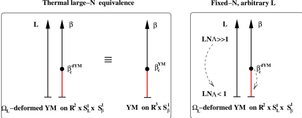
Figure 1: (Left) At N = \infty , the thermodynamics of the deformed and undeformed Yang-Mills theories are equivalent. (Right) Unlike pure Yang-Mills, the deformed theory has, at finite N , a semi-classical domain (defined by LNA \lesssim 1 ) where the confinement-deconfinement transition is analytically calculable.
