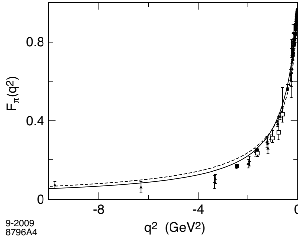
Fig. 4. Space-like scaling behavior for F_\pi(Q^2) as a function of q^2 . The continuous line is the prediction of the soft-wall model for \kappa = 0.375 GeV. The dashed line is the prediction of the hard-wall model for \Lambda_{\text{QCD}} = 0.22 GeV. The triangles are the data compilation from Baldini et al. , [26] the filled boxes are JLAB 1 data [27] and empty boxes are JLAB 2 data. [28]
