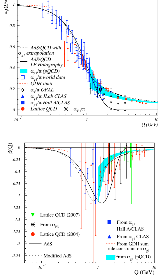
Fig. 7. (a) Effective coupling from LF holography for \kappa = 0.54 GeV compared with effective QCD couplings extracted from different observables and lattice results. (b) Prediction for the \beta -function compared to lattice simulations, JLab and CCFR results for the Bjorken sum rule effective charge.
