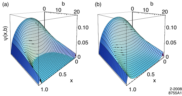
Fig. 3. Pion light-front wavefunction \psi_\pi(x, \mathbf{b}_\perp) for the AdS/QCD (a) hard-wall ( \Lambda_{QCD} = 0.32 GeV) and (b) soft-wall ( \kappa = 0.375 GeV) models.
