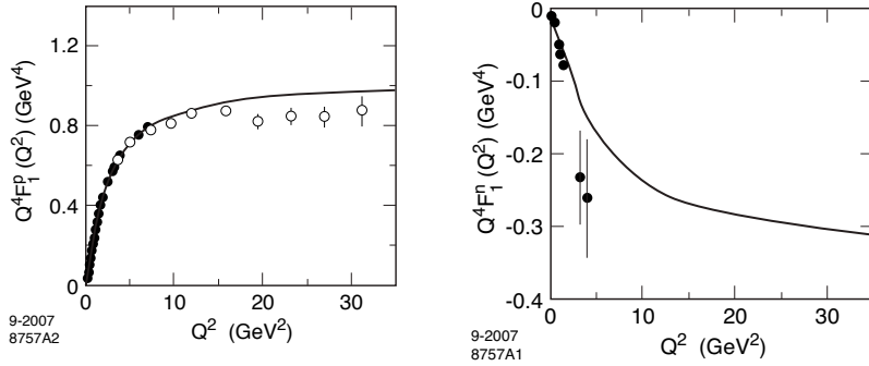
Fig. 6. Predictions for Q^4 F_1^p(Q^2) and Q^4 F_1^n(Q^2) in the soft wall model for \kappa = 0.424 GeV. [119]
