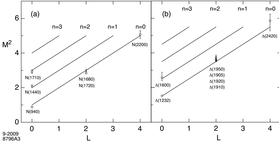
Fig. 5. 56 Regge trajectories for the N and \Delta baryon families for \kappa = 0.5 GeV
