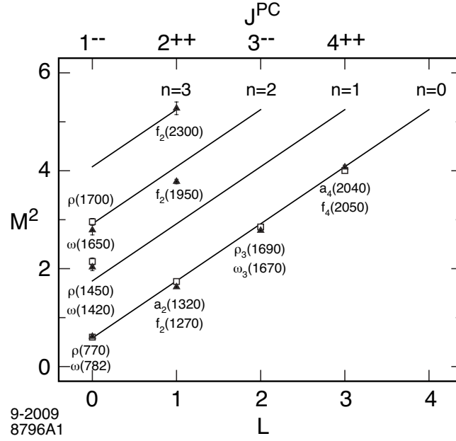
Fig. 2. Regge trajectories for the I=1 \rho -meson and the I=0 \omega -meson families for \kappa = 0.54 GeV.
