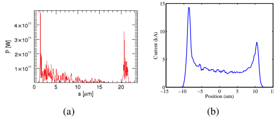
Figure 7: Genesis simulation showing power as a function of longitudinal bunch position (left). The peak power occurs in the current spikes (right). For this simulation, the spikes had emittances of 0.6 \mu\text{m} .
