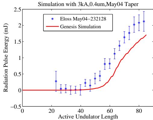
Figure 11: Post-saturation FEL pulse energy for a taper with nearly 9 MeV final average electron energy loss. Genesis simulations for a 0.4\mu\text{m} emittance beam agree well, but have slightly less FEL power.
