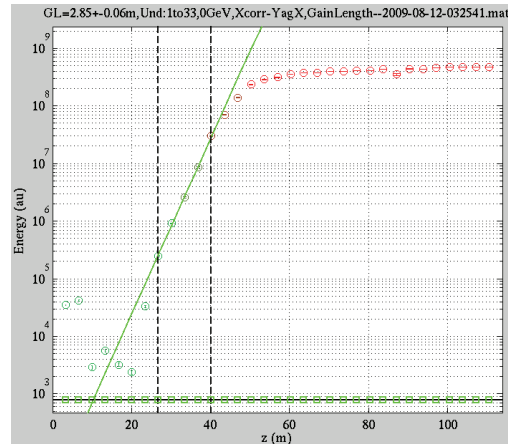
Figure 5: Gain length of 2.85 \pm 0.06 m taken at 13.6 GeV using the dipole corrector method. The high power levels of the first two data points are due to a secondary FEL spot as seen in Fig. 3.
