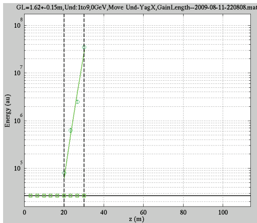
Figure 8: Gain length of 1.62 \pm 0.15 \text{ m} taken at 4.7 GeV using the undulator pull method.
