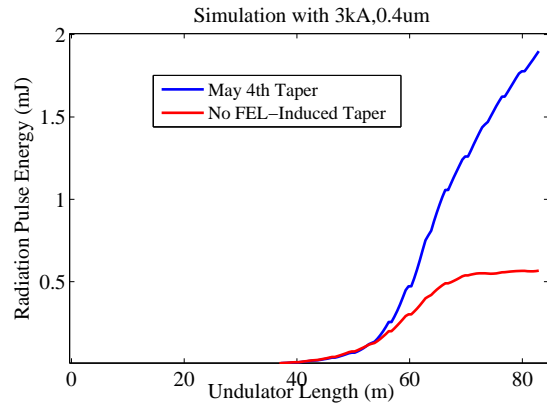
Figure 13: Simulation results show a post-saturation taper increasing the FEL output by greater than a factor of 3.
