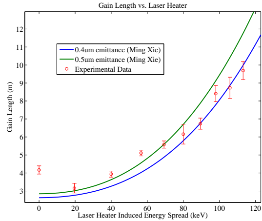
Figure 9: Gain length as a function of energy spread following the laser heater. Ming Xie scaling shown for 0.4, 0.5 \mu\text{m} emittances. We note the increased gain length with no laser heating (0 keV), hinting at the importance of the laser heater to suppress the microbunching instability. The nominal heater value induces a 20 keV energy spread.
