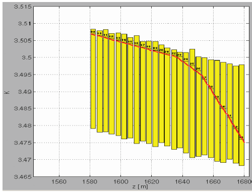
Figure 10: Experimentally-optimized undulator taper (red line) that yielded an FEL-induced average electron energy loss of nearly 9 MeV. Yellow boxes show available range of taper for each undulator.
