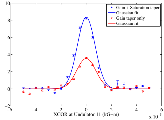
Figure 12: Measured FEL-induced electron energy loss as a function of dipole kick at undulator 11. The addition of a saturation taper can increase the FEL output by a factor of greater than 2.
