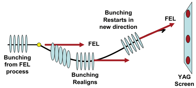
Figure 4: The bunching can either realign or restart from shot noise, creating secondary FEL spots. In this cartoon, down corresponds to positive X on the YAG screen
