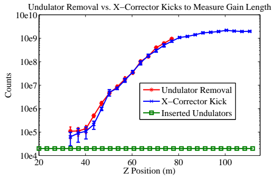
Figure 2: Gain lengths measured with both the undulator removal and dipole corrector kick methods. Distances are for total undulator length and do not include the breaks between segments.
