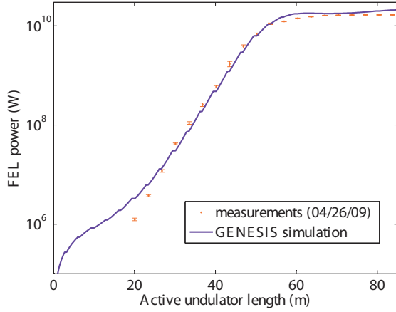
Figure 6: A gain length measurement of 3.3 m agrees well with Genesis simulations for a beam with 0.4 \mu\text{m} emittance.
