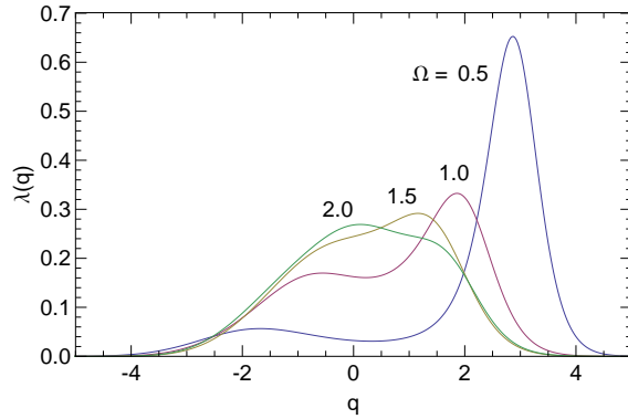
FIG. 2: For the Q = 1 resonator, the Haussinski solution at threshold, for the cases \Omega = 0.5, 1.0, 1.5, 2.0 . Note that the bunch head is to the right.
