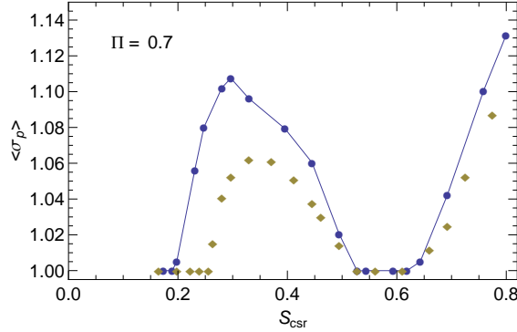
FIG. 5: For shielded CSR with \Pi = 0.7 , the value of \sigma_p , averaged over 400 synchrotron periods, \langle \sigma_p \rangle , as given by the VFP simulations. The case of nominal damping \beta = 1.25 \times 10^{-3} is given by blue circles (connected by straight lines), the case of \beta = 2.5 \times 10^{-3} by olive diamonds.
