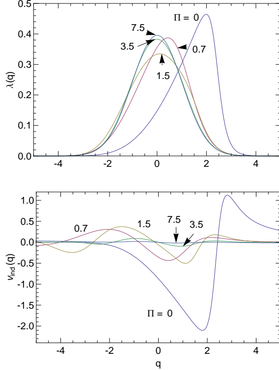
FIG. 4: Haässinki solution at threshold and wake induced voltage for shielded CSR, for the cases \Pi = 0.0, 0.7, 1.5, 3.5, 7.5 . Note that bunch head is to the right.
