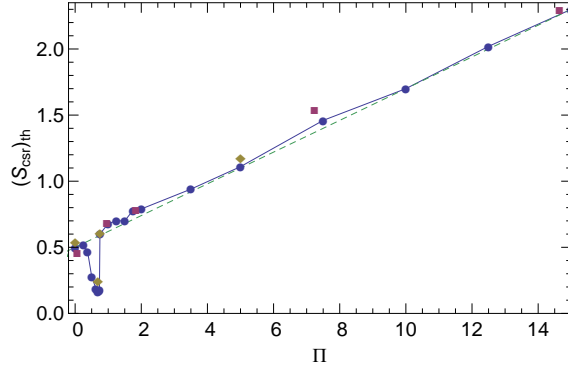
FIG. 3: For the CSR wake, threshold value of S_{\text{csr}} vs. shielding parameter, \Pi = \rho^{1/2}\sigma_{z0}/h^{3/2} . Symbols give results of the VFP solver (blue circles), the LV code (red squares), and the VFP solver with twice stronger radiation damping (olive diamonds).
