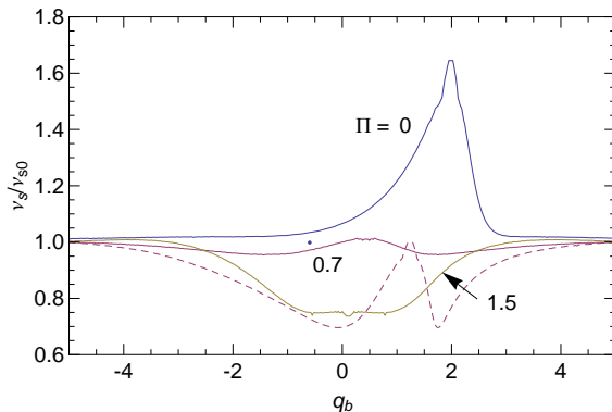
FIG. 7: Shielded CSR: incoherent tune at threshold due to the distorted potential well, as function of position of maximum excursion, q_b , for cases \Pi = 0, 0.7 , and 1.5 . The dashed curve is explained in the text below.
