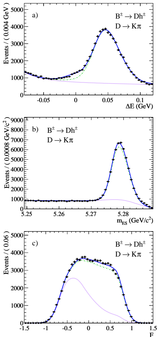
FIG. 5: Projections of (a) \Delta E , (b) m_{ES} , and (c) \mathcal{F} variables of the fit to the B^\pm \rightarrow Dh^\pm , D^0 \rightarrow K^-\pi^+ flavor mode. No requirements are put on the PID of the track h from the B decay and on the fit variables not plotted. See caption of Fig. 2 for line definitions.
