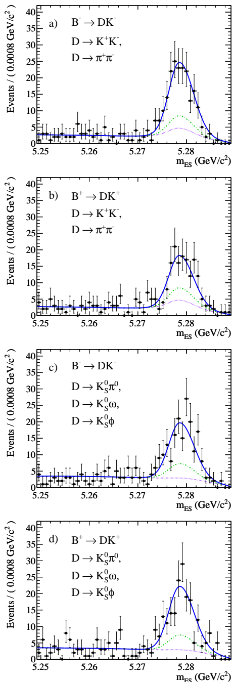
FIG. 3: m_{ES} projections of the fits to the data, split into subsets of definite CP of the D candidate and charge of the B candidate: a) B^- \rightarrow D_{CP+}K^- , b) B^+ \rightarrow D_{CP+}K^+ , c) B^- \rightarrow D_{CP-}K^- , d) B^+ \rightarrow D_{CP-}K^+ . We show the subsets of the data sample in which the track h from the B decay is identified as a kaon. See caption of Fig. 2 for line definitions. Only a subrange of the whole fit range is shown in order to provide a closer view of the signal peak.
