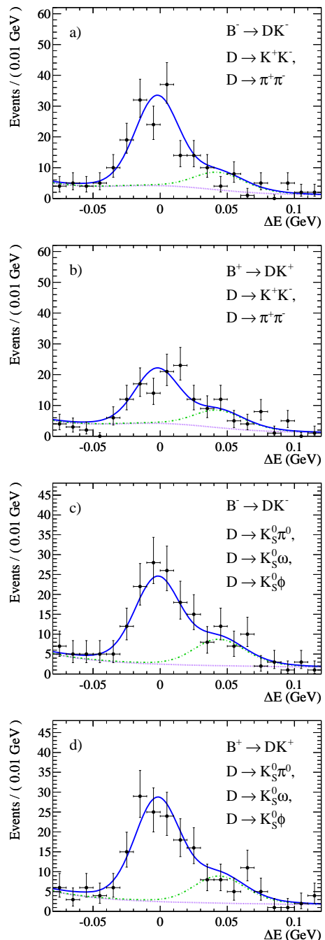
FIG. 2: \Delta E projections of the fits to the data, split into subsets of definite CP of the D candidate and charge of the B candidate: a) B^- \rightarrow D_{CP+}K^- , b) B^+ \rightarrow D_{CP+}K^+ , c) B^- \rightarrow D_{CP-}K^- , d) B^+ \rightarrow D_{CP-}K^+ . The curves are the full PDF (solid, blue), and B \rightarrow D\pi (dash-dotted, green) stacked on the remaining backgrounds (dotted, purple). The region between the solid and the dash-dotted lines represents the B \rightarrow DK contribution. We show the subsets of the data sample in which the track h from the B decay is identified as a kaon. We require candidates to lie inside the signal-enriched region defined in Sec. IV, except for the plotted variable.
