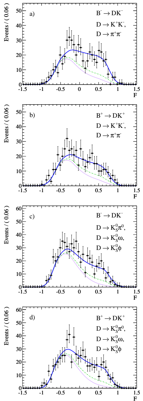
FIG. 4: \mathcal{F} projections of the fits to the data, split into subsets of definite CP of the D candidate and charge of the B candidate: a) B^- \rightarrow D_{CP+}K^- , b) B^+ \rightarrow D_{CP+}K^+ , c) B^- \rightarrow D_{CP-}K^- , d) B^+ \rightarrow D_{CP-}K^+ . We show the subsets of the data sample in which the track h from the B decay is identified as a kaon. See caption of Fig. 2 for line definitions.
