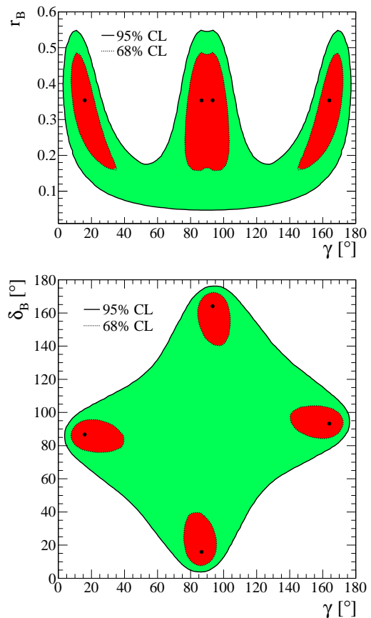
FIG. 7: Contours at 68% (dotted, red) and 95% (solid, green) 2-dimensional CL in the (\gamma, r_B) and (\gamma, \delta_B) planes. See also the caption of Fig. 6 regarding symmetries.
