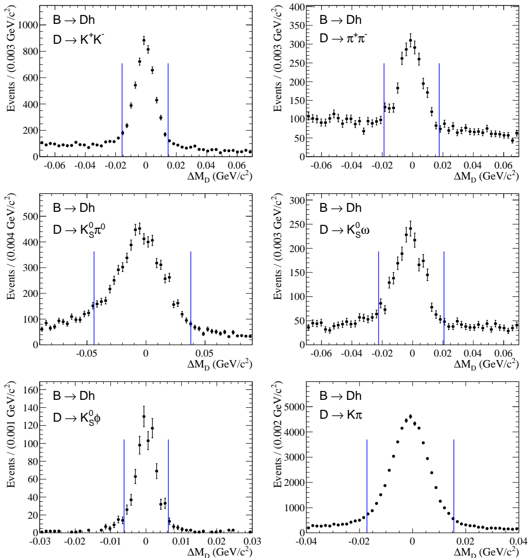
FIG. 1: Distributions of the difference between the D candidate's invariant mass and the nominal D^0 mass [30], as measured in the B^\pm \rightarrow Dh^\pm samples. All selection criteria described in Section IV, except that on the D invariant mass M_D , have been applied. In addition we reduce the background by requiring the fit variables to satisfy m_{ES} > 5.27 \text{ GeV}/c^2 , \Delta E > -0.05 \text{ GeV} , and \mathcal{F} > -0.25 . The \Delta M_D selection requirements are depicted by the vertical lines.
