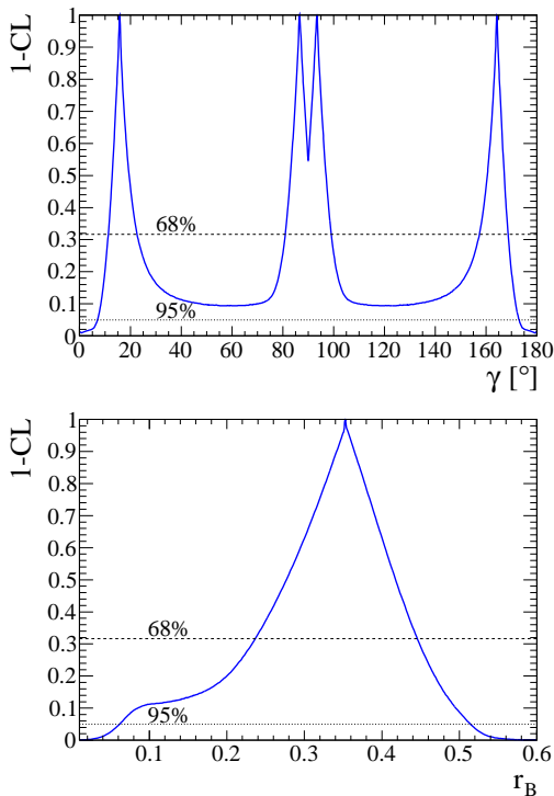
FIG. 6: 1-CL as a function of \gamma (top) and r_B (bottom). Both statistical and systematic uncertainties are taken into account. For the angle \gamma , the plot is identical in the range [180^\circ, 360^\circ] . The horizontal lines show the 68% CL (dashed) and the 95% CL (dotted). Due to the symmetry of Eqns. 3 and 4 the plot for the strong phase \delta_B is identical to the one for \gamma .
