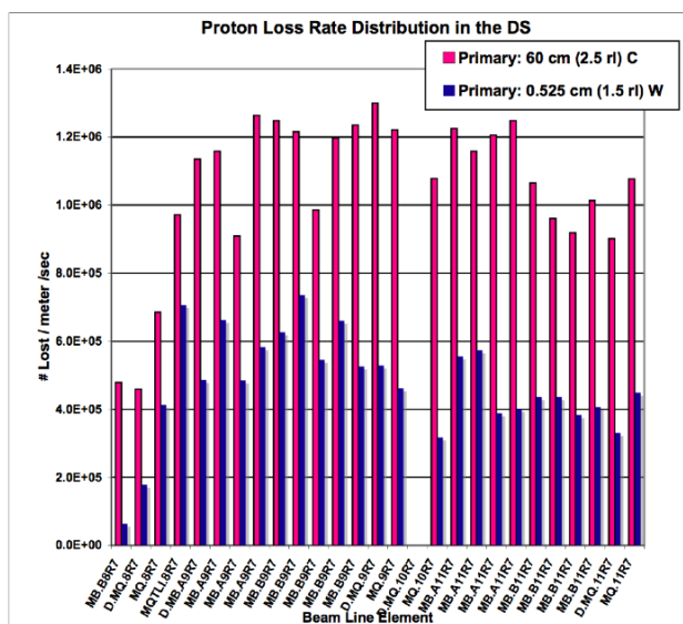
Figure 1. Loss rate/meter on cold magnets in the dispersion suppressor for carbon primary (red) and tungsten primary (blue). In this plot the four long dipoles are divided into sections. In total there are approximately twice as many losses with a carbon primary.
