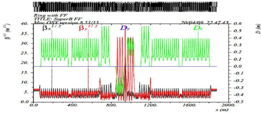
Figure 3: HER optical functions with spin rotator insertions.
