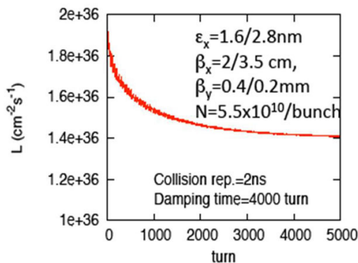
Figure 1: SuperB strong-strong simulation (BBSS).
