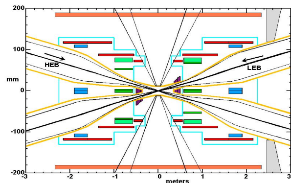
Figure 2: SuperB Interaction Region.
