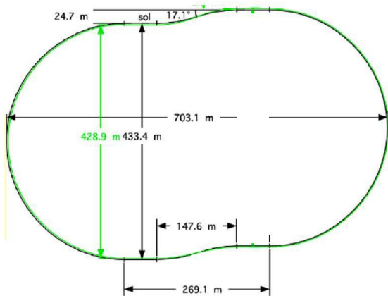
Figure 4: SuperB layout with spin rotators.
