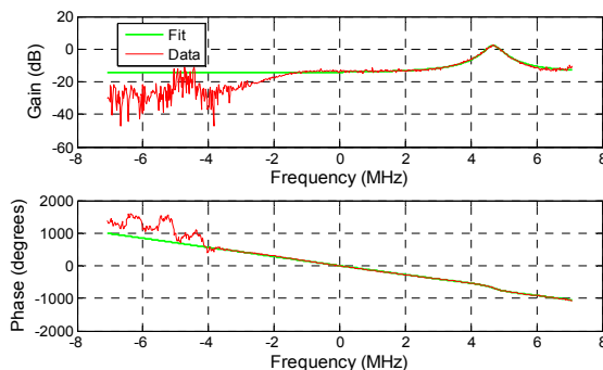
Figure 2: Klystron transfer function : Measured and fitted model
