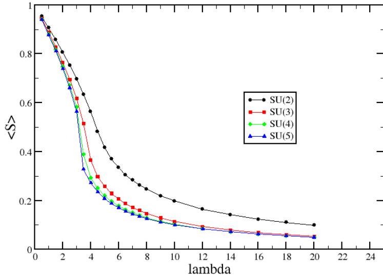
Figure 2: Plaquette action in the quenched theory vs 't Hooft coupling
