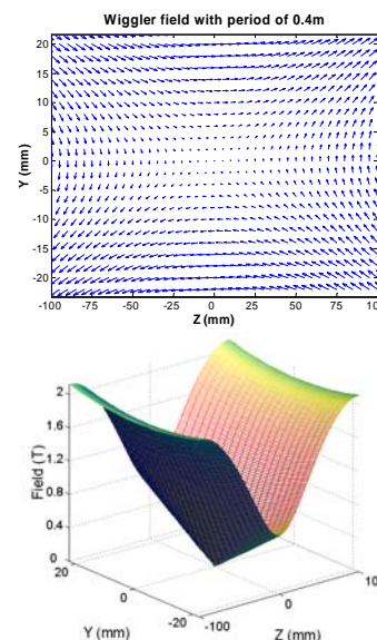
Figure 1: Wiggler field distribution (top) and field strength in vertical-longitudinal plane.
