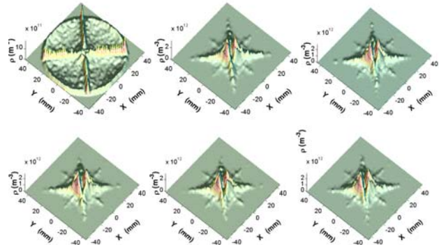
Figure 7: Evolution of electron cloud during the train gap, frames separated by \Delta t=70 ns . Parameters used for simulation: Bunch length 17.24 mm, bunch current 1.0 mA, bunch spacing 14 ns, field gradient 9.2 T/m , peak SEY 2.0, energy at peak SEY 310 eV, photon flux 0.21 photons/m/particle, reflectivity 20%.
