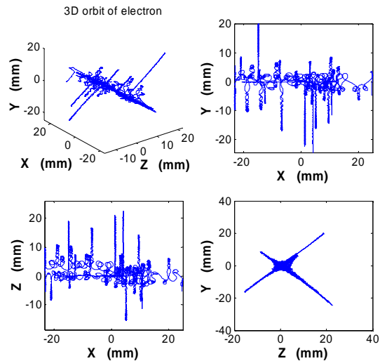
Figure 4: Example of an electron trajectory, which shows how the electron passes through the beam chamber horizontally.
