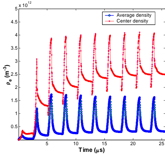
Figure 5: Electron build-up in the quadrupole magnet with a field gradient of 9.2T/m .
