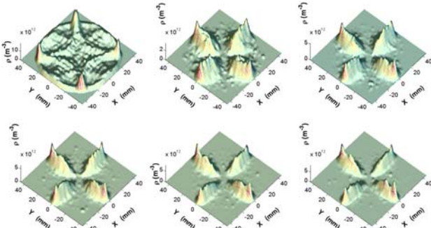
Figure 5: Electron build-up in the quadrupole magnet with a field gradient of 9.2T/m .
