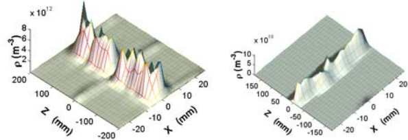
Figure 3: Electron cloud distribution in horizontal and longitudinal plane for 10% (left) and 0% (right) photon reflectivity.
