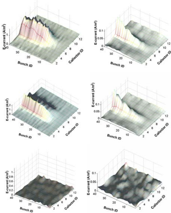
Figure 2: Simulated electron flux in RFAs of CESRTA wiggler: peak field region (top), zero vertical field region (bottom) and the region in between (middle) for a bunch current 1.5mA (Left) and 0.45mA (Right). The collector is installed on the top of the beam chamber and the collector ID shows the horizontal position, collector 7 th is the central collector.
