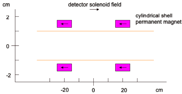
Figure 6: Axially magnetized PM cylinders near IP.
