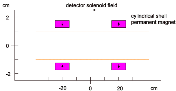
Figure 8: Radially magnetized PM cylinders near IP.
