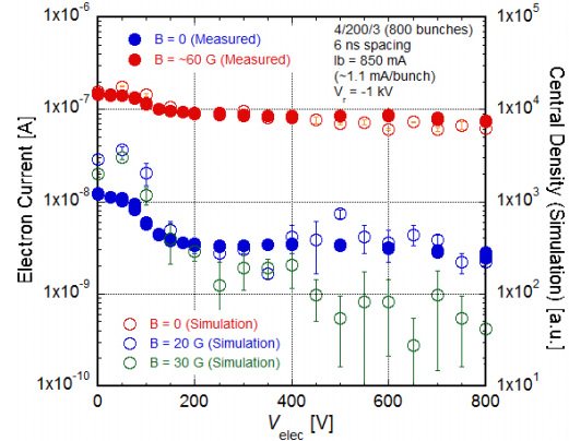
Figure 7: Behaviours of measured electron currents against the applied voltage for B = 0 and \sim 60 G. The calculated central electron densities for B = 0, 20 and 30 G are also plotted for comparison.
