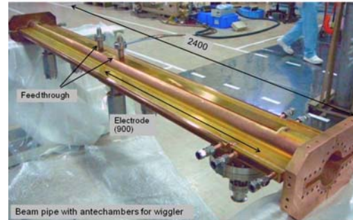
Figure 4 (a): Beam pipe with antechambers for wiggler magnets, where two clearing electrode are prepared at top of the beam channel.
