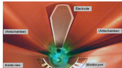
Figure 4 (b): Inside view of a beam pipe with antechambers and clearing electrodes. An electron monitor is placed at the bottom of an electrode.
