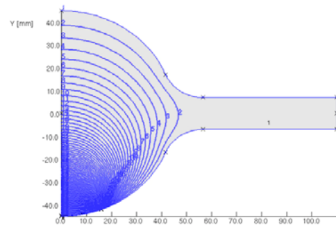
Figure 5: Calculated equipotential lines due to an electrode at the bottom of a beam pipe with antechamber.
