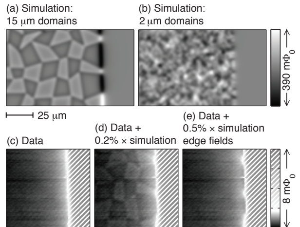
FIG. 5: (a,b) Simulated scans of a quasiperiodic domain structure in \text{Sr}_2\text{RuO}_4 . The MS results are extended to z = 2.0 \mu\text{m} using eq. 1, then averaged over a 3.2 \mu\text{m} -diameter pick-up coil. (c) Observed signal, from Fig. 3(c). (d,e) Observed signal plus a scale factor times the simulation. In (e), domain wall contributions are removed.
