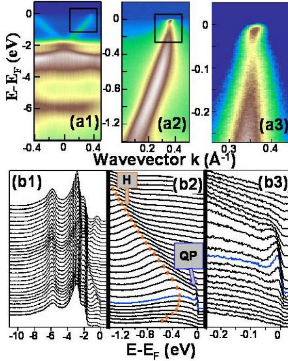
Figure 1 Data collected along the (0,0)-(\pi,\pi) nodal direction at various magnifications. (a1), (b1), Image plot and EDC of the valence band around the \Gamma point. The Mn e_g states show a \approx 1.8 eV dispersion, \approx 0.4 eV wider than that predicted by LDA calculations 8 (Lin, H., Sahrakorpi, S., Barbiellini, B. & Bansil, A., personal communication). (a2), Magnification of the box in (a1) and stacks of EDC of the e_g band, showing the break-up of the spectral weight into a small quasiparticle peak which crosses E_F at a Fermi wavevector k_F \approx 0.37 \text{ \AA}^{-1} , and a rapidly dispersing broad peak (the hump, H). (a3), Magnification of the box in (a2) and relative EDC (b3). The data have been collected at 20 K with photon energy h\nu = 42 eV and the light polarization vector lying in the sample plane.
