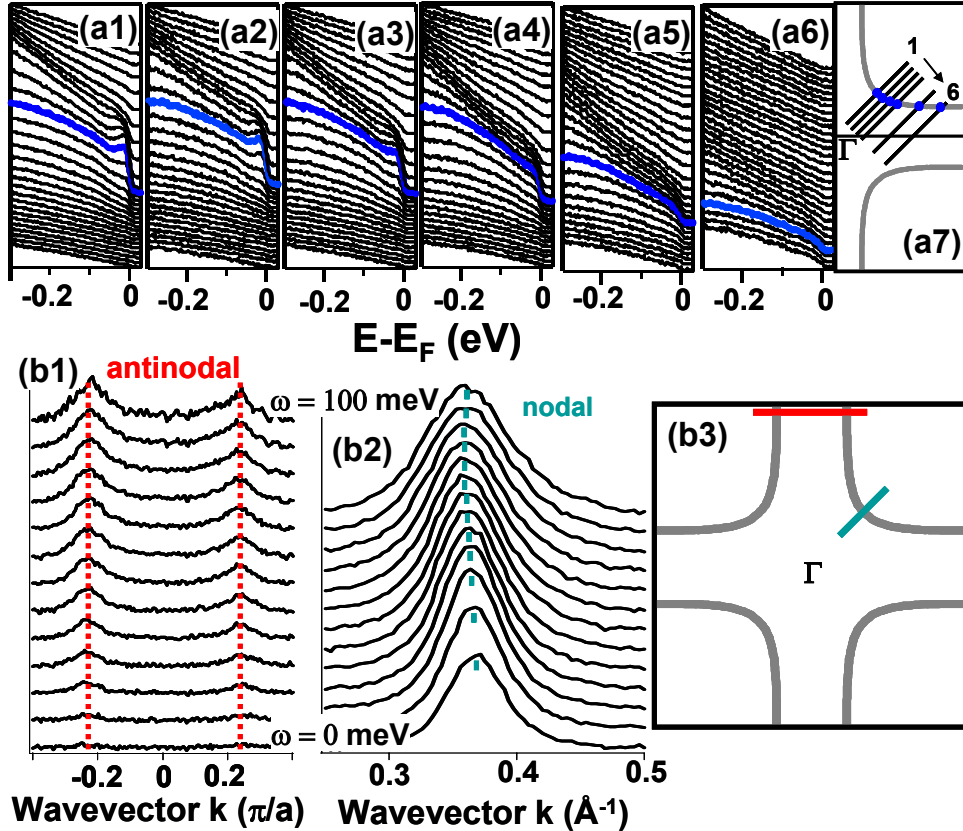
Figure 4 Nodal-antinodal dichotomy in momentum space. (a1)-(a6), EDC corresponding to the cuts shown in (a7). The spectral weight of the well-defined quasiparticle peak rapidly loses intensity while moving away from the nodal direction. (b1), MDC spectra for the antinodal; (b2), nodal cuts shown in (b3). The presence of quasiparticle peaks along the nodal direction and their absence along the antinodal sections of the Fermi surface is not related to an anisotropic distribution of spectral intensity due to matrix element effects. This is evident from Fig. 3, which shows that there are regions in the parallel Fermi surface sections that contain strong spectral intensity, but do not yield well-defined quasiparticle peaks such as those along the node.
