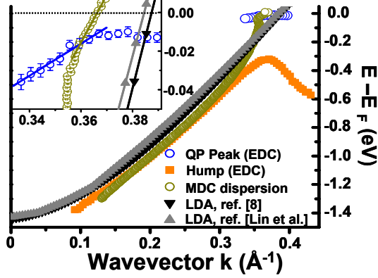
Figure 2 Dispersion of the e_g band. Aside from a rigid shift, there seems to be a good correspondence for energies higher than \approx 300 - 400 meV between the e_g band dispersions calculated with LDA 8 (Lin, H., Sahrakorpi, S., Barbiellini, B. & Bansil, A., personal communication) and extracted with the MDC analysis of the data shown in Fig. 1(a2). Also shown are the positions of the broad peak (hump) and the quasiparticle peak determined from the EDC shown in Figs 1(b2) and 1(b3). The inset shows the magnification of the region close to the Fermi level crossing. The solid lines indicate the results of the fittings. If not shown, the error bars are smaller than the symbol's size. The MDC analysis for energies approaching E_F leads to an S-shaped dispersion with two kinks near 50 and 100 meV. This S-shaped dispersion is an artefact resulting from the way the MDC analysis handles the Englesberg-Schrieffer two-poles solution 19 , namely the distribution of spectral weight for energies ranging from \approx 50 meV to the maximum of the broad hump peak. Nevertheless, the energy scale revealed by the 50 meV kink is still meaningful, as it marks the asymptotic energy separating the coherent quasiparticle peak from the hump, as also shown in Fig. 1(a3).
