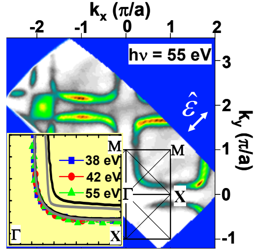
Figure 3 Fermi surface topology. The Fermi surface has been determined by integrating the spectral weight in a \pm 50 meV window around E_F of spectra excited with photons of 55 eV. Reducing the integration window to \pm 10 meV results in the same spectral weight distribution. The momentum distribution of spectral weight is strongly affected by the photon energy and especially the experimental geometry, as a result of the impact that symmetry has on the matrix elements 2 . According to LDA calculations, the Fermi surface topology consists of a small electron pocket derived from 3z^2 -like states centred at the \Gamma point and x^2-y^2 -derived hole pockets centred at the M point and split into two by the hybridization between the bilayers 8 (Lin, H., Sahrakorpi, S., Barbiellini, B. & Bansil, A., personal communication). We found that (data not shown) the small electron pocket centred at \Gamma is enhanced when the photon polarization vector is perpendicular to the sample plane, unlike in the cases shown here, for which the light polarization vector lies in the sample plane directed along the nodal direction (white arrow). This geometry was nonetheless used because it gives better exposure of the spectral weight at E_F . To better quantify the Fermi surface, we made use of the MDC analysis, which identifies as Fermi wavevectors ( k_F ) the maximum positions of the momentum distribution of spectral weight at E_F . The result is shown in the inset, where the Fermi surface contour extracted with the MDC analysis of data collected at three different photon energies is compared to the LDA calculations from ref. 8 (black line) and the work of Lin, H., Sahrakorpi, S., Barbiellini, B. & Bansil, A. (personal communication) (grey line). Despite an extensive search involving the use of different photon energy and/or experimental geometries, we observed only the x^2-y^2 band closest to the \Gamma point, which tracks the LDA prediction extremely well, giving us confidence that our data are truly representative of the LSMO compound.
