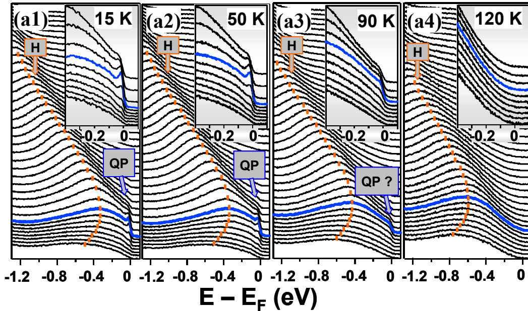
Figure 5 Temperature-dependent evolution of the nodal quasiparticle. The data have been collected along the (0,0)-(\pi,\pi) nodal direction with photon energy h\nu = 42 eV and light polarization vector lying in the sample plane. Note the very small changes with temperature of the broad peak (hump, H) as opposed to the dramatic changes of the quasiparticle peak (insets). The quasiparticle peak - visible in (a1) and (a2) - becomes hard to track at T = 90 K = 0.75 T_C (a3) and is undetectable at the Curie temperature T_C = 120 K (a4), which is concomitant with a metal-insulator transition between a low-temperature ferromagnetic-metallic ground state and a high-temperature paramagnetic-insulating phase. To ensure reproducibility of the data and exclude the occurrence of any surface damage during the measurements, the spectra have been collected by both increasing and decreasing the temperature.
