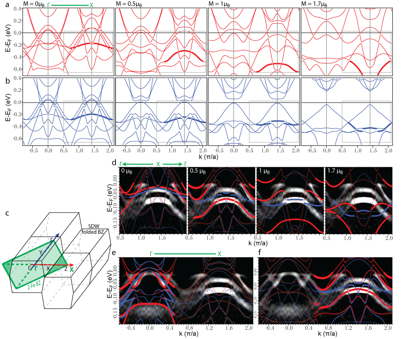
FIG. 7: Comparison of BaFe 2 As 2 band dispersions with fixed-moment LDA. (a) LDA calculations of bands along \Gamma -X-Z in the folded SDW BZ (corresponding to \Gamma -X of the paramagnetic BZ, see (c)) with magnetic moments fixed at different values. Thicker segments trace the trend that bands shift in energy with increasing moment. (b) Same as in (a) except for the direction along \Gamma -Y- \Gamma in the folded SDW BZ. (c) 3-D BZ schematic. Green denotes 1st BZ in the paramagnetic state that is probed under our experimental setup. In the SDW state, the base-centered orthorhombic structure corresponds to a BZ (black) staggered in k_z in one direction. The original equivalent \Gamma -X directions in the paramagnetic state now becomes \Gamma -X-Z (red arrow) and \Gamma -Y- \Gamma (blue arrow) directions. Averaging over magnetic domains under the synchrotron beam spot leads to a mixture of signals from the \Gamma -X-Z and \Gamma -Y- \Gamma directions. (d) LDA ( k_z = 0 ) with various fixed magnetic moments overlaid on experimental data around X point in the \Gamma -X direction, with contribution from both \Gamma -X-Z (red) and \Gamma -Y- \Gamma (blue) directions. All LDA bands are shifted up in energy by 0.12 eV and renormalized by a factor of 3. (e) The best match (LDA with M = 0.5 \mu_B ) overlaid on band dispersion along the \Gamma -X cut, unshifted but renormalized by a factor of 3 to fit with bands around \Gamma . (f) same as (e) except with LDA shifted up in energy by 0.12 eV and renormalized by the same factor of 3 to fit with bands around X.
