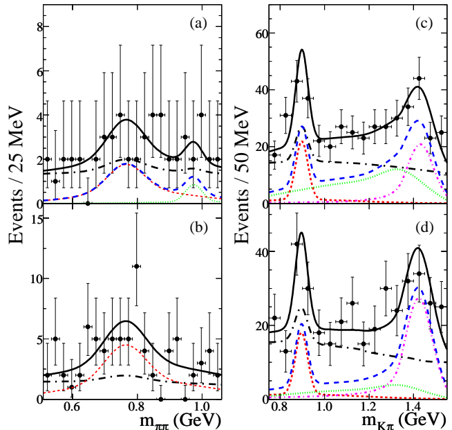
FIG. 2: B -candidate m_{\pi\pi} projections for (a) \eta'\rho^0/\eta'f_0 , (b) \eta'\rho^+ , and m_{K\pi} for (c) \eta'K^{*0} , (d) \eta'K^{*+} . Color online: the solid curve is the fit function, black long-dash-dotted is the total background, and the blue dashed curve is the total signal contribution. In (a) we separate the \rho^0 component (red dashed) from the f_0 (green dotted). In (c,d) we separate the K^*(892) (red dashed), the (K\pi)_0^* (green dotted), and K_2^*(1430) (magenta dot-dashed) components.
