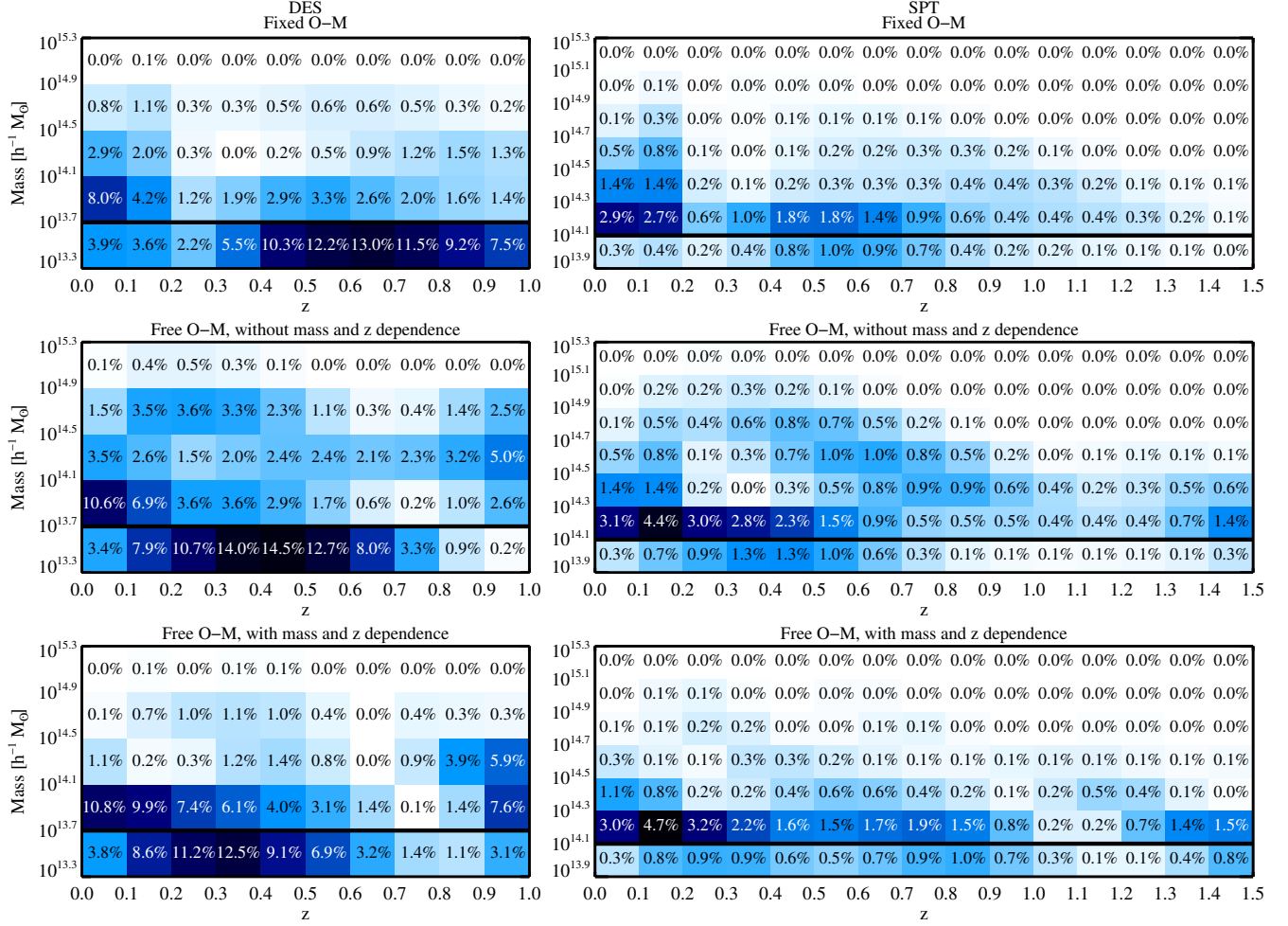
FIG. 4.— Relative importance of f_i in different mass (vertical axes) and redshift (horizontal axes) bins for a DES-like survey ( left ) and an SPT-like survey ( right ). The number in each bin reflect the percentage improvement in the FoM that results from tightening the prior on the mass function in that bin (from 10% to 1% for DES and from 30% to 3% for SPT), and the shading scales linearly with the number. The top panels correspond to a fixed observable–mass relation with known mean and scatter; the middle panels correspond to a free observable–mass relation in which the mean and scatter are self-calibrated but are not mass or redshift dependent; and the bottom panels correspond to a free observable–mass relation that has mass- and redshift-dependent mean and scatter specified by the parameters of Equation (7). The horizontal thick line shows the observable threshold; the low-mass bins near this threshold are the most important because of the high cluster counts in these bins. The patterns in the redshift dimension are largely determined by a combination of the CMB prior, the clusters counts, and the degeneracy between f_i and scatter.
