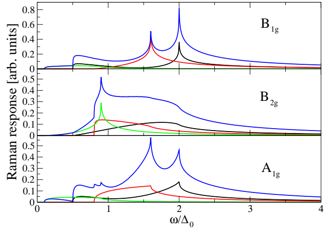
FIG. 7: Same as Fig. 6 but for r_\beta = 0.6 .
