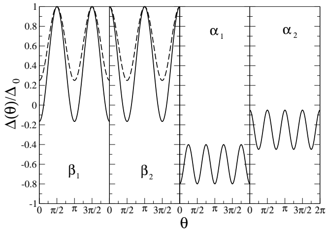
FIG. 2: The anisotropic energy gaps around the 4 Fermi surface sheets as a function of angle \theta shown in Fig. 1. For the \beta sheets, the solid line is for r_\beta = 1.4 and the dotted line r_\beta = 0.6 (see Eq. 14).
