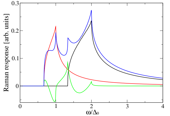
FIG. 5: The screened A_{1g} Raman response for 2 bands with \Delta_{1,2}(\theta) proportional to (1 + r \cos(4\theta))/(1 + r) with r = 0.2 , and the maximum gap on Fermi surface 1 equal to \Delta_0 and on Fermi surface 2 equal to \Delta_0/2 . (black = screened A_{1g} for band 1, red = screened A_{1g} for band 2, green = mixing term, blue = total response.)
