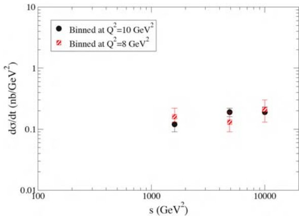
FIG. 13: The H1 data from Ref. [51] for t = -0.8\text{GeV}^2 .
