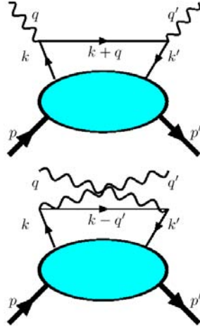
FIG. 2: The handbag and crossed-handbag diagrams convoluting the hard scattering amplitude together with a soft Generalized Parton Distribution.
