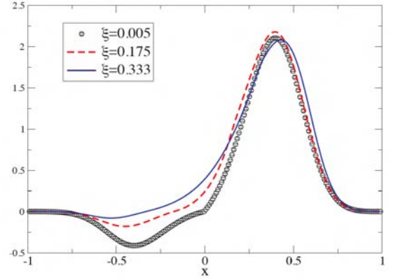
FIG. 10: The H(x, \xi, t) GPD at fixed -t = 1 GeV 2 with the parameters discussed in text.
