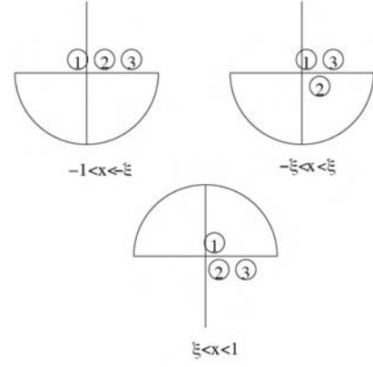
FIG. 8: Integration over the \tilde{k}^- variable in Eq.(78) is performed in the complex plane where location of the poles of the integrand is determined by the denominators in Eq.(79). Location of these poles is in agreement with Ref. [43]. For x < \xi , H(x < -\xi) receives a contribution from the \hat{s} -channel and for x < \xi , H(x > \xi) is determined by the \hat{u} -channel.
