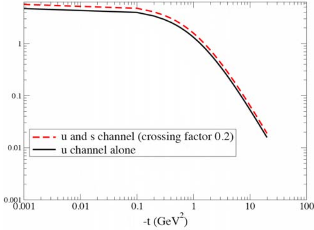
FIG. 9: The F_{1/x} form factor in the perturbative diquark model. At large -t the form factor is power-law suppressed.
