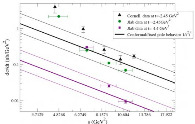
FIG. 12: The Cornell data from Ref. [12] is replotted for the fixed value of t = -2.45 \text{ GeV}^2 . For comparison we also show recent JLab data from Ref. [52].
