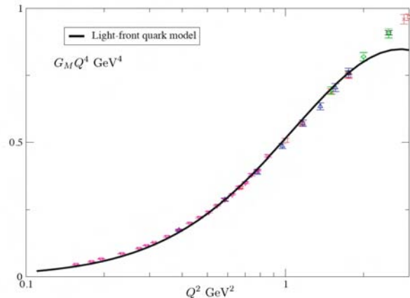
FIG. 4: Proton Sachs form factor in the impulse approximation with light-front Gaussian wave function from Eq.(71). Since this approximation excludes the hard, one-gluon exchange component (as opposed to Fig. 3), the form factor representation can only be trusted until about 3 GeV ^2 .
