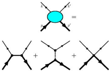
FIG. 15: A simple, perturbative model for a two-body scattering amplitude, given by the sum of an s -channel, t -channel and contact interaction.
