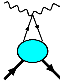
FIG. 1: The local coupling of two photons to a quark yields a fixed pole, a real and constant contribution to the Compton amplitude. In scalar electrodynamics this fixed pole is easy to recognize –it originates from the seagull coupling. For spin 1/2 quarks, one needs to pick up an instantaneous (on the light-front) Z-diagram component of the handbag diagram, as shown in Eq.(6).
