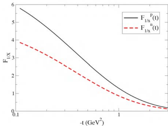
FIG. 5: The 1/x form factor of the proton and neutron in the valence light-front quark model. The ratio is equal to 2/3 arising from the ratio of quark electric charges. Parameters are as in Fig. 3
