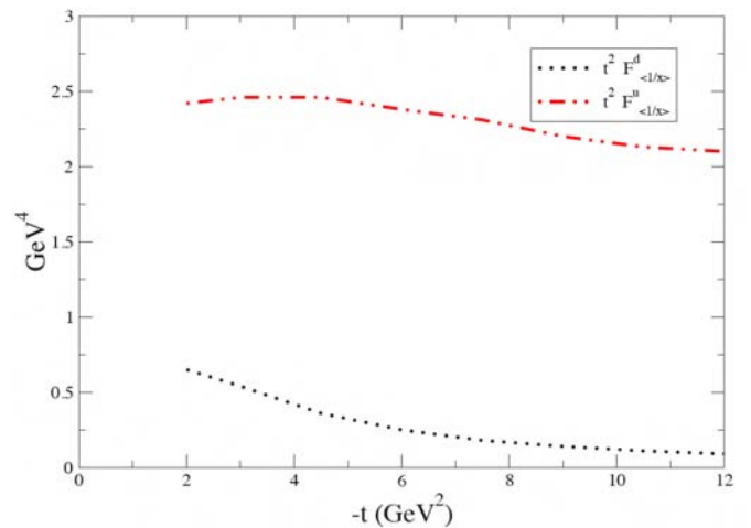
FIG. 7: An evaluation of the 1/x form factors of the proton has been carried out in the Gaussian light-front constituent quark model, valid for large -t . The authors present the flavor-separated form factors from a set of GPD's fit to a number of conventional Dirac and Pauli form factors. Computer data from Ref. [40].
