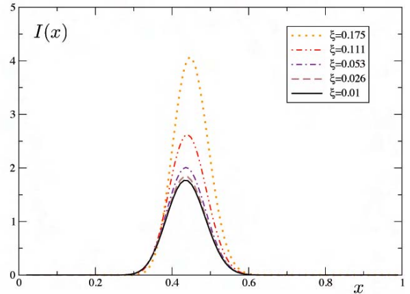
FIG. 6: We plot the unintegrated handbag amplitude given in Eq.(73). The area under the left-most curve is smaller than all others, and tags the J = 0 fixed pole.
