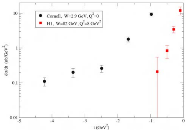
FIG. 11: The t dependence of the real Compton and deeply virtual Compton scattering cross sections from Cornell [12] and H1 [50] experiments, respectively.
