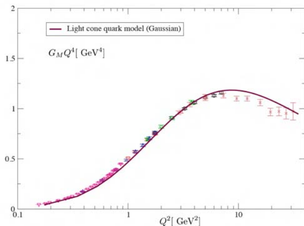
FIG. 3: Proton Sachs form factor in the impulse approximation with light-front Gaussian wave function of Eq.(71) and one-gluon exchange. The parameters employed are m = 250 MeV and b = 1.2 GeV ^{-2} . Data are taken from Ref. [33].
