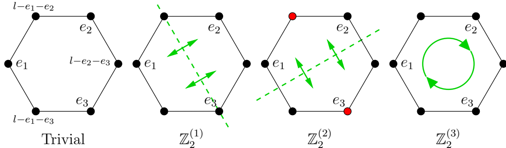
Figure 8: The trivial and the three order-2 automorphisms of the graph of (-1) -curves on \mathcal{B}_3 .
