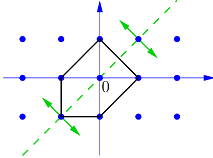
Figure 6: Symmetry of the toric polytope defining \mathcal{B}_1 .
