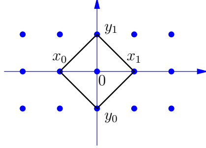
Figure 5: The toric polytope defining \mathbb{P}^1 \times \mathbb{P}^1 .
