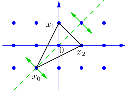
Figure 4: Symmetry of the toric polytope defining \mathbb{P}^2 .
