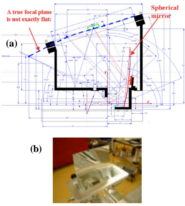
Fig. 3. (a) FDIRC prototype with a spherical mirror and bar. A calculated focal plane is not exactly flat, but not far from flat approximation for shown range of dip angles. The picture also shows the bar coordinate system. (b) A real picture of the mirror in the prototype.
