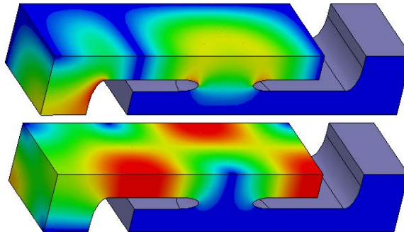
Figure 2: Half geometry of one period from mid-cell to mid-cell. The top image shows the electric field pattern and the bottom one the magnetic field pattern for one of the two symmetric, out-of phase modes.
