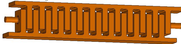
Figure 4: Example of a 24 cell, 15.75 cm zipper structure.
