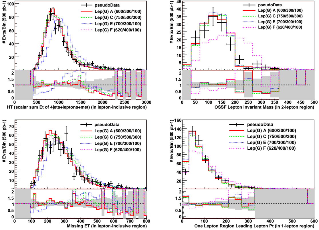
FIG. 6: Two variables that constrain the kinematics are H_T and the \ell^+\ell^- invariant mass in dilepton events (top left and right, respectively). \cancel{E}_T and single-lepton p_T have similar sensitivity (bottom left and right). Over the pseudo-data (black error bars), we show Lep(G) models at four parameter values, all from Table III: the best fit A (red, solid), and mass variations C, E, and F as described in the plot legends. Model C (the green dashed line) is globally consistent with both the data and model A, although it has a rather different mass spectrum; E and F are constrained by H_T and m_{\ell^+\ell^-} , respectively.
