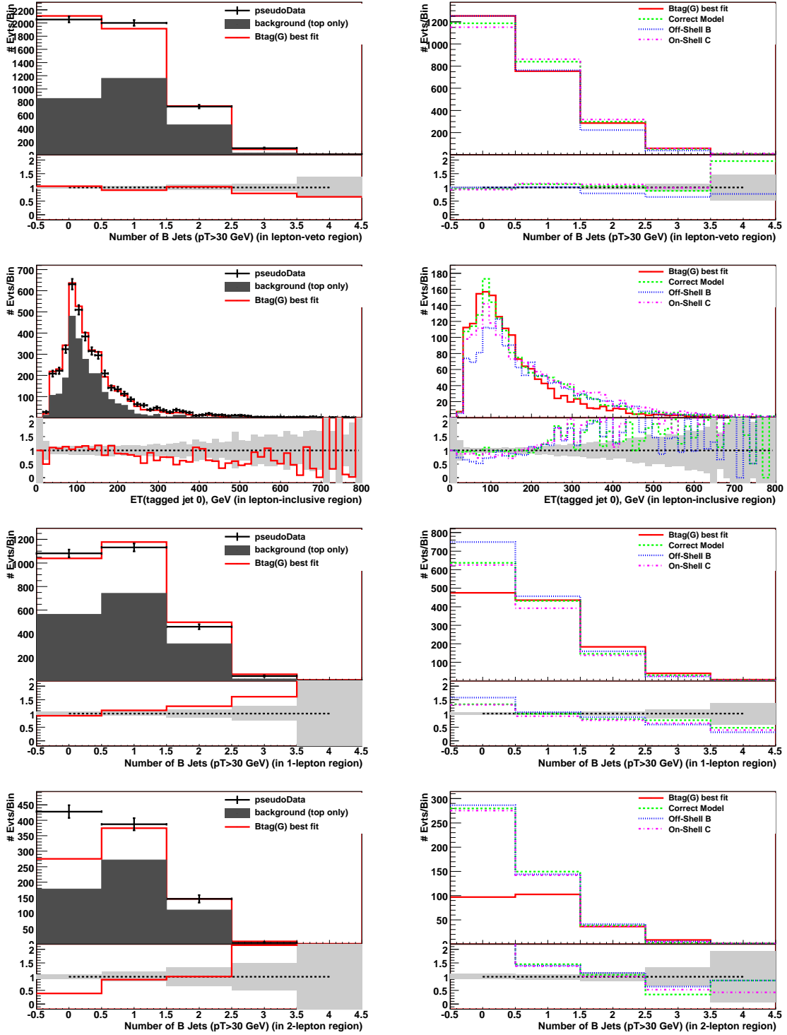
FIG. 23: Left: Comparisons of Data, corresponding to 500\text{pb}^{-1} with t\bar{t} backgrounds superimposed, to Simplified Model Btag(G) (exclusive lepton fit) with parameters M_G = 700 GeV, M_{LSP} = 100 GeV, \sigma = 11.8\text{pb} , B_{uu} = 35.4\% , B_{bb} = 2.8\% , B_{tt} = 61.8\% . Right. Comparison of the same simplified model to SUSY models off-shell B, and on-shell C, as well as the correct model. Error bars have been suppressed on the model comparisons, but they can be taken as statistical. From top to bottom, the distributions shown are: number of b -jets and p_T of hardest b -jet (lepton-inclusive region), number of b -jets in 1-lepton and 2-lepton regions.
