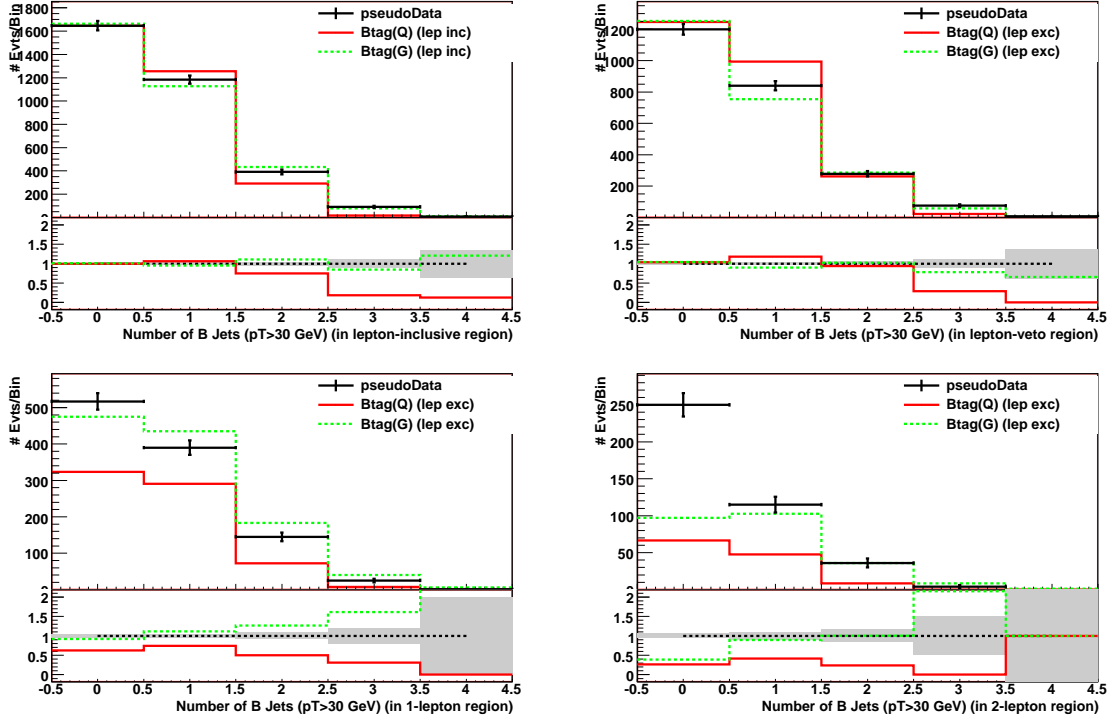
FIG. 20: Example 2: b -jet count distributions for the lepton inclusive, 0, 1, and 2 lepton regions. Note that B_{\text{tag}}(G) provides a better overall description of these signatures. Also note that the lepton exclusive fits, in which W 's from top-channels are used to account for leptons, fail to account for all the lepton in the 0 b -jet regions. This is strong evidence for lepton channels beyond those that may accompany any third generation channels.
