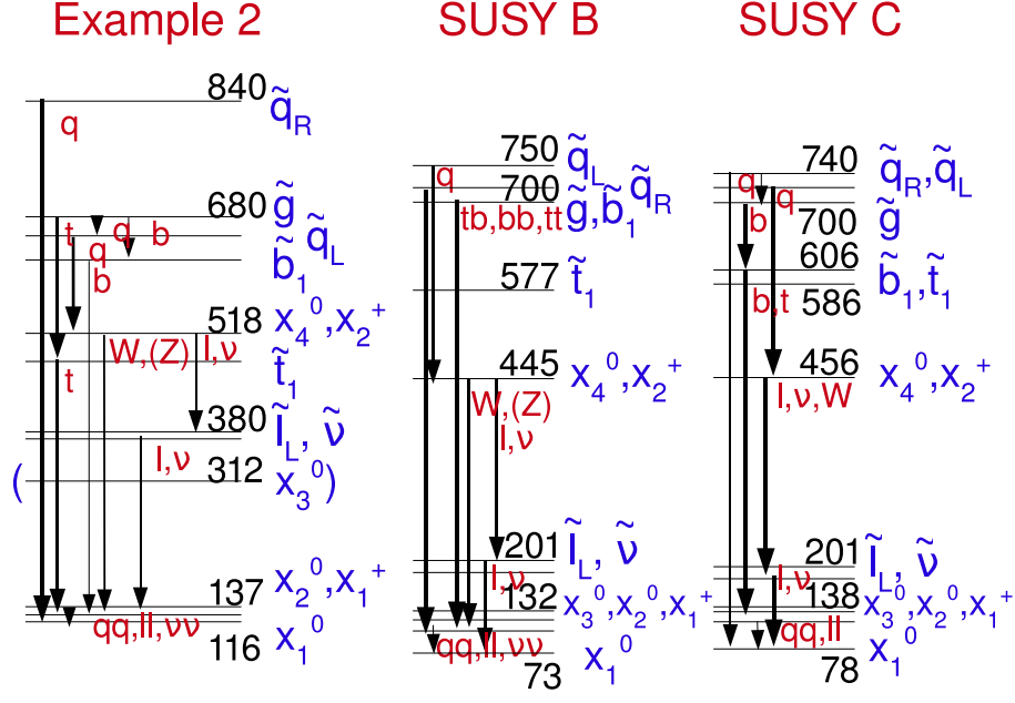
FIG. 24: Left: Spectrum cartoon for the model used in Example 2 (parameters in Appendix B 3 b). Right: Spectra for SUSY models offB and onC used in the comparison in sec. VID 2 (parameters in Appendix B 3 c)
