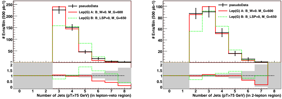
FIG. 5: Jet counts (in 0- and 2-lepton regions) between “data” (error bars) and the simplified model Lep(G) with parameter set A ( B_W = 0 , red solid line) or B ( B_{LSP} = 0 , green dashed) from Table III.
