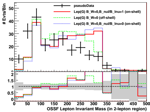
FIG. 18: Example 2: On- and off- shell Lep(G) fits comparing the structure of the OSSF di-lepton invariant mass.
