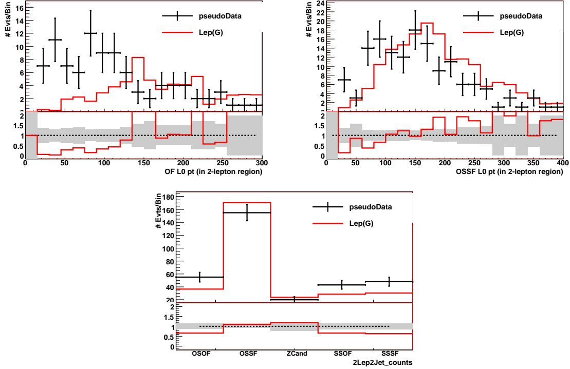
FIG. 15: Comparisons of di-lepton kinematics and counts between the “data” (error bars) and simplified model Lep(G) (red), in a case where the data has a high fraction of WW , WZ , ll + W , and \ell\nu + W decay modes. A good diagnostic for this in the Lep(Q/G) fits is an excess of opposite flavor di-leptons relative to single lepton or same flavor events. Typically in such cases, there is also a difference in the lepton kinematics between opposite flavor and same flavor. See sec. VB
