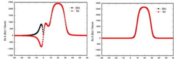
Fig. 2: Typical axial magnetic field profiles in the gun region for high charge (left) and low charge (right).
