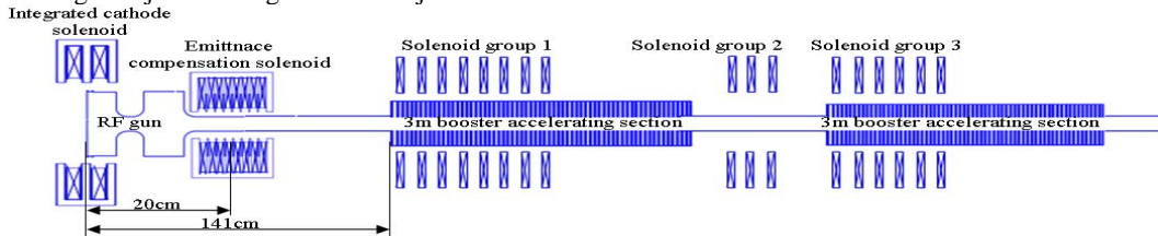
Fig. 1: Schematic layout of the photoinjector.
