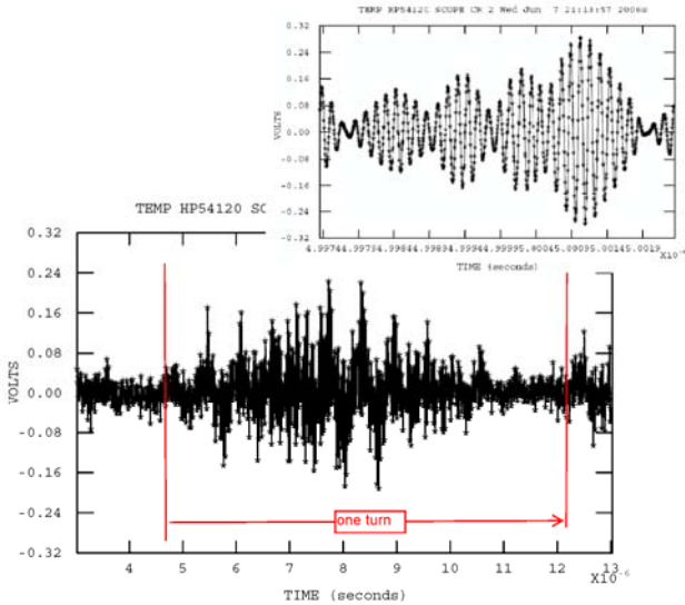
Figure 3: Oscilloscope signal from the antenna in a multi-bunch two beam operation.
