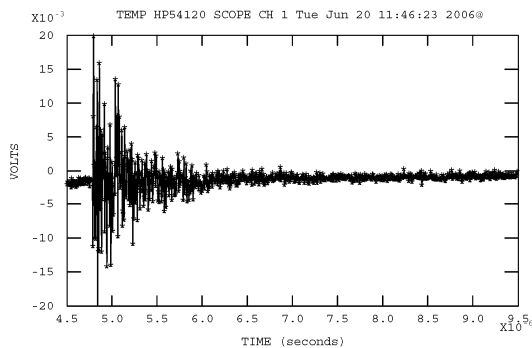
Figure 4: Oscilloscope signal from the antenna in a single bunch operation.
