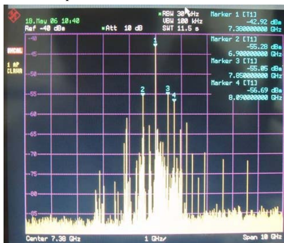
Figure 2: HOM spectrum, measured in a multi-bunch operation.
