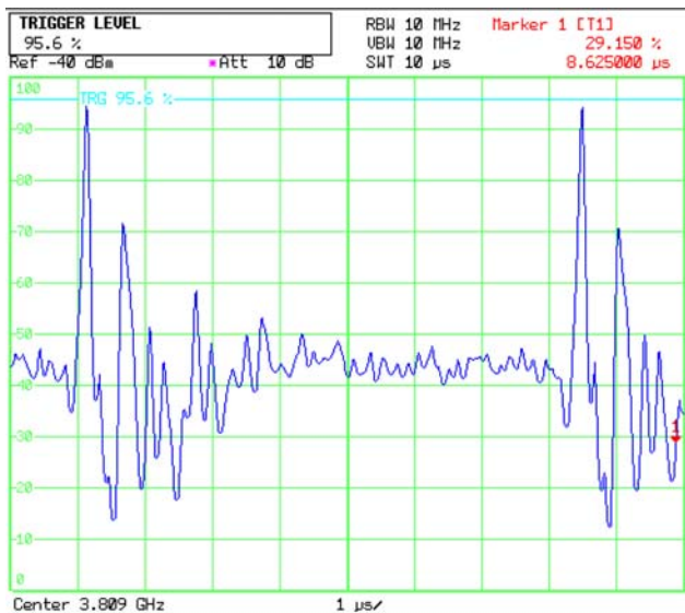
Figure 9: Transient at f=3.8 GHz.
