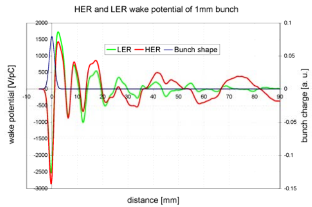
Figure 9: HER and LER wake potentials of 1 a mm bunch, which were used in the calculation of the bunch lengthening
