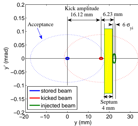
Figure 9: Schematic of phase space at injection.
