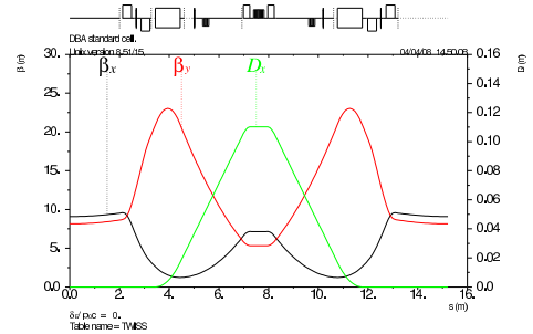
Figure 2: Optics functions in one DBA cell.
