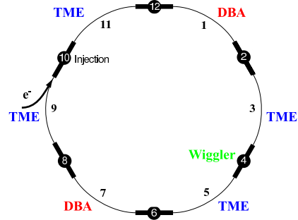
Figure 1: PEP-X layout with 2 DBA and 4 TME arcs.
