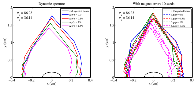
Figure 8: Dynamic aperture without errors (left) and with multipole field errors based on the specifications of PEP-II magnets for 10 random settings (right).
