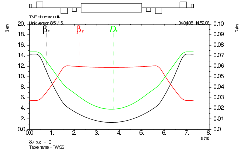
Figure 3: Optics functions in one regular TME cell.
