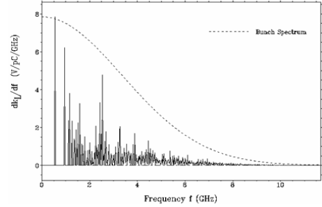
Figure 8: Spectrum for 10mm bunch in Geo-1.
