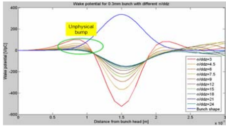
Figure 2: ABCI simulation results for 0.3\text{mm} bunch.
