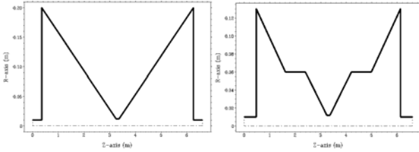
Figure 7: Alternative geometries of ILC Interaction Region chamber (Geo-2 & Geo-3).
