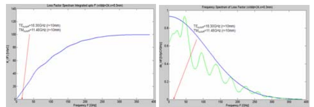
Figure 6: Long range wake and spectrum ( \sigma_z=0.3\text{mm} ).
