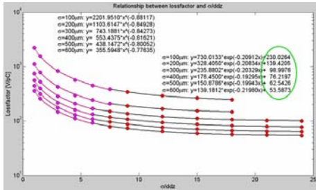
Figure 3: Simulation for different \sigma_z with different \sigma_z/ddz .
