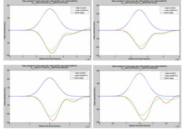
Figure 4: Comparison of MAFIA 2D and ABCI.
