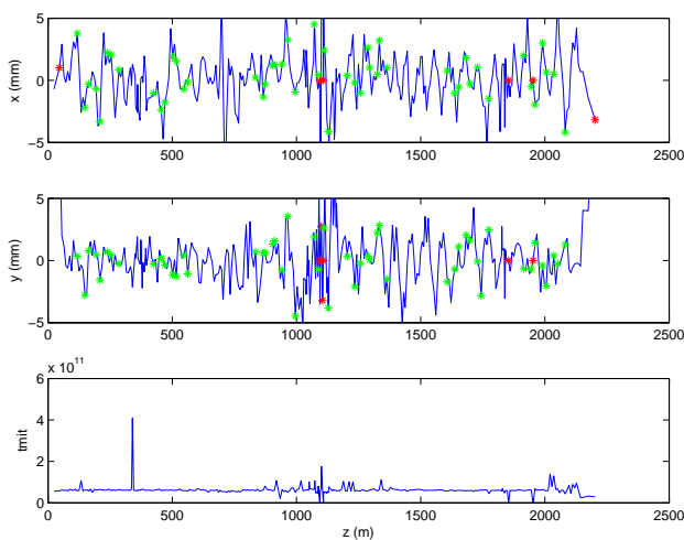
Figure 1: Live orbit data from the LER in PEP II. The blue trace represents the orbit measurement from the older system. The red stars are units flagged as showing bad data. The green stars are the orbit measurements with the new system.
