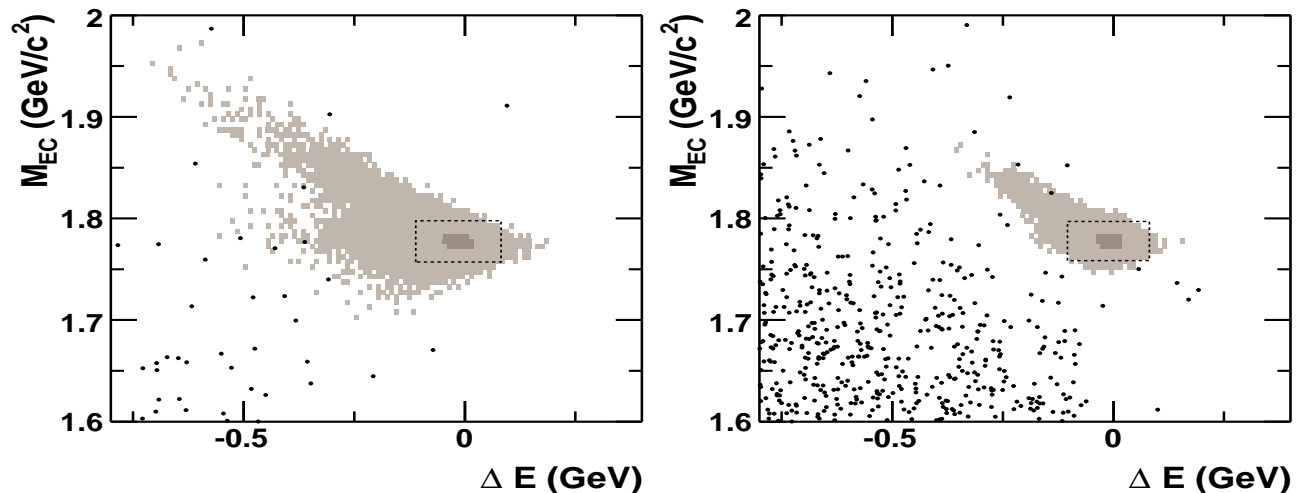
FIG. 1: The selected candidates (dots) inside the large box region of the m_{\text{EC}}-\Delta E plane for \tau^\pm \rightarrow e^\pm\omega (left plot) and \tau^\pm \rightarrow \mu^\pm\omega (right plot) decays. The \pm 3\sigma signal box is shown by a dashed rectangle. The dark and light shading indicates contours containing 50% and 90% of the selected MC signal events, respectively. The signal box contains 67% of the selected MC signal events for \tau^\pm \rightarrow e^\pm\omega and 77% for \tau^\pm \rightarrow \mu^\pm\omega decay.
