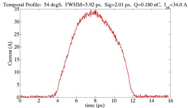
Figure 3: Temporal dist. of 34-A e^- beam measured with the transverse RF deflector upstream of BC1 ( \sigma_t \approx 2.0 ps).
