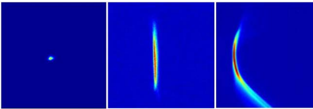
Figure 4: Screen-1 image with RF deflector OFF (left) and ON (middle), for measuring sliced emittance. Screen-2, after a bend (right), shows longitudinal phase space.
