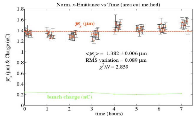
Figure 6: Hor. projected emittance measured over 8 hours.
