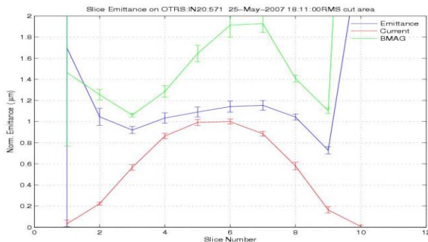
Figure 5: Time-sliced horizontal emittance measurement on OTR screen using quad-scan at 0.2 nC and 1.5-mm cathode spot radius. Each time-slice is about 1 ps wide.
