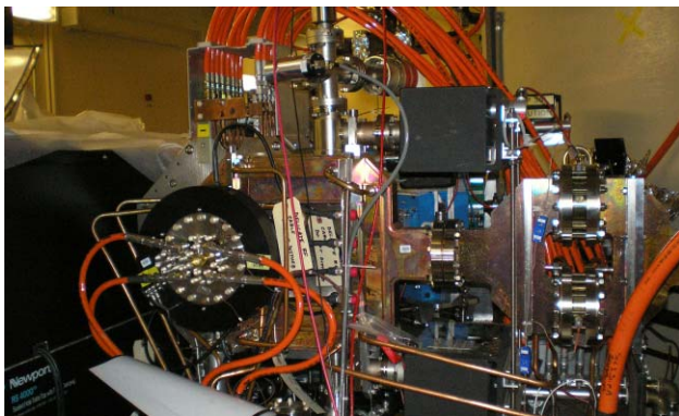
Figure 2: The LCLS Gun-1 installed. View is from rear of gun with dual RF feed at right and cathode assembly toward left. The cathode flange has cooling lines and black bucking coil connected. The drive laser launch optics and virtual cathode camera are in black box at left.
