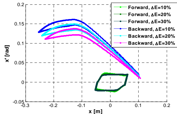
Figure 2: Forward and backward tracked phase spaces do not overlap, indicating top-off is safe.
