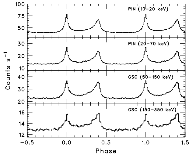
Fig. 39. Folded light curves of the Crab pulsar in four energy bands, obtained as a sum of the 64 PIN diodes or the 16 Well units. The observed counts are folded at the pulse period, and are shown for two pulse phases.
