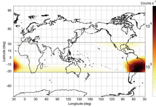
Fig. 20. The flux map of cosmic-ray and trapped particles measured by the PIN-UD count.
