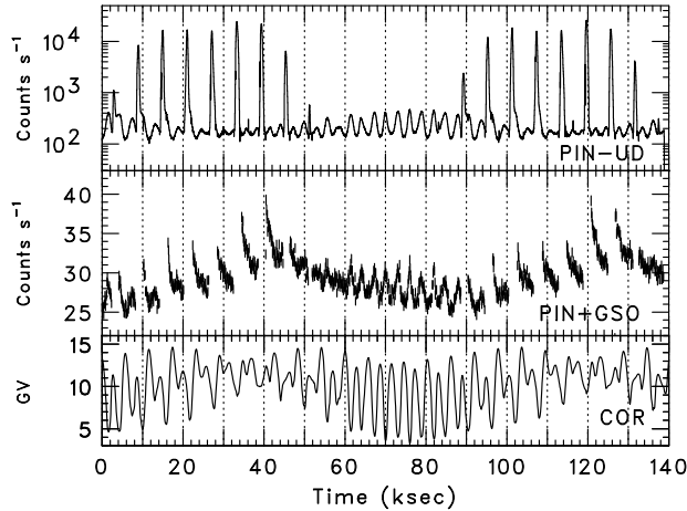
Fig. 19. Typical light curves of the PIN-UD counting rate summed over the 16 units ( top ), “cleaned” events from PIN and GSO ( middle ), and the cut-off rigidity ( bottom ), obtained from \sim 1.5 days observation of a blank sky field.
