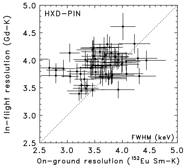
Fig. 4. Comparison between the energy resolutions of the PIN diodes measured on-ground and in-orbit, by use of ^{152}\text{Eu} isotope ( \text{Sm-K}_{\alpha 1} : 40.1 keV) and the Gd- \text{K}_{\alpha 1} (43.0 keV) line, respectively.
