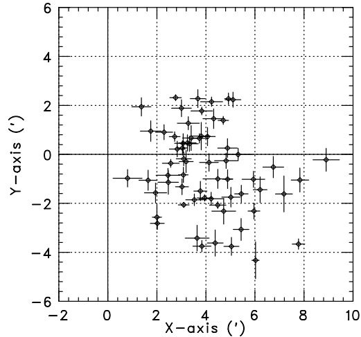
Fig. 33. A summary plot of the distribution of individual optical axes of the 64 fine collimators.
