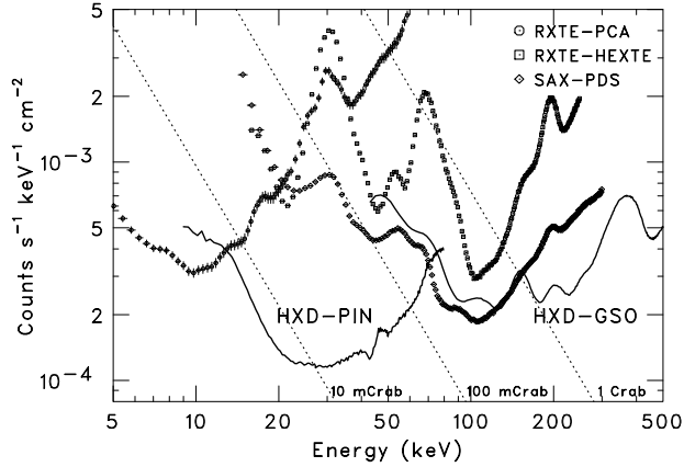
Fig. 31. The in-orbit detector background of PIN/GSO, averaged over 2005 August to 2006 March and normalized by individual effective areas. For comparison, those of the RXTE-PCA, RXTE-HEXTE, and BeppoSAX-PDS are also shown. Dotted lines indicate 1 Crab, 100 mCrab, and 10 mCrab intensities.
