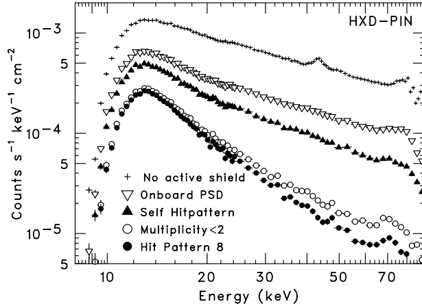
Fig. 9. The background spectra summed over the 64 PINs, acquired under various reduction conditions (see text). They are normalized by the total geometrical area of the 64 PIN diodes.
