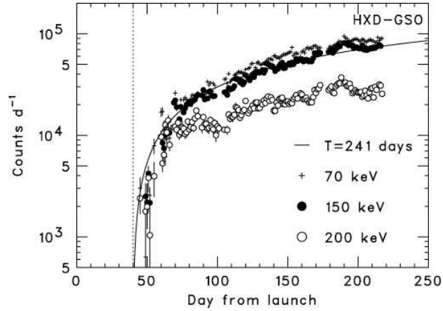
Fig. 28. Light curves of the peak counts of the tree prominent EC-decay isotopes, compared with the predicted evolution curve for a half-life of 241 days. The difference spectra are obtained by subtracting the in-orbit background taken at 40 days, as indicated by a dotted line.
