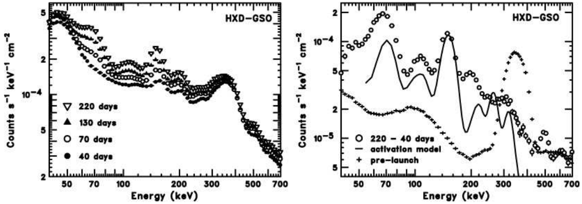
Fig. 27. ( Left: ) An evolution of averaged GSO-NXB spectra during the first half year after the launch. Each observation has an exposure longer than a day. ( Right: ) A difference GSO-NXB spectrum between 40 and 220 days after the launch (open circles), compared with the estimated long-nuclides spectrum (smooth curve). The pre-launch intrinsic background is also shown (crosses).
