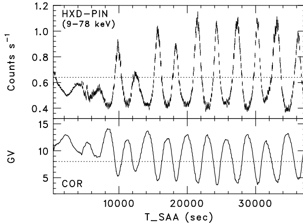
Fig. 23. A light curve of the PIN-NXB folded with T_SAA in an energy range of 9-78 keV ( top ), and a plot of cut-off rigidity obtained as an average for each T_SAA ( bottom ).
