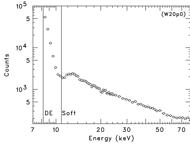
Fig. 7. A typical background spectrum of one PIN. Two vertical lines indicate the LD level applied in HXD-DE, and the energy threshold used in the processing software.
