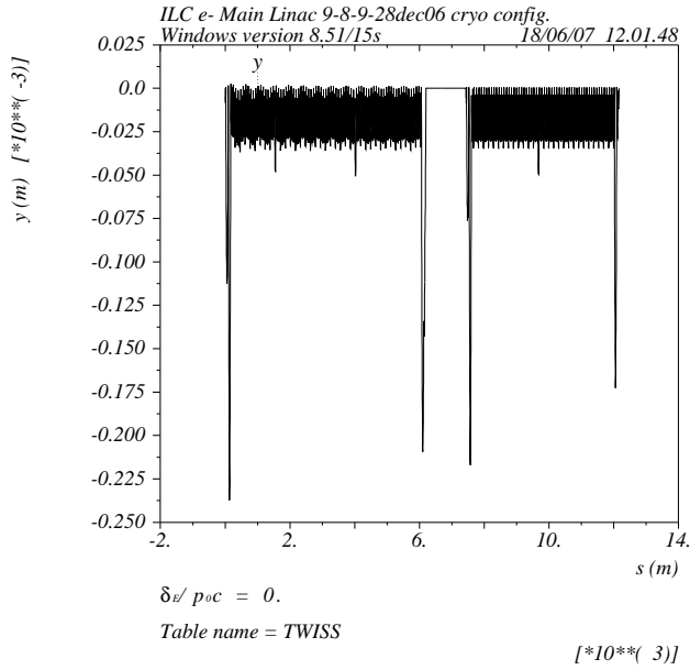
Figure 4: Vertical orbit in the curved linac.
