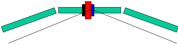
Figure 3: Curvature implementation. Green blocks are cryomodules, black block is the BPM, red - quadrupole, blue - corrector, black line is the beam orbit.
