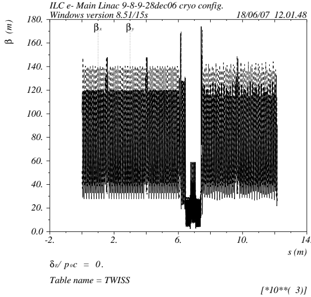
Figure 2: Beta-functions in the electron linac.
