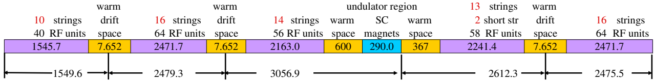
Figure 1: Layout of cryogenic components.
