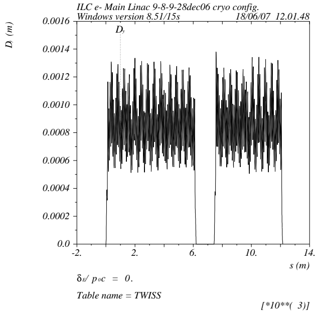
Figure 5: Vertical dispersion in the curved linac.
