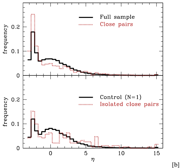
FIG. 6.— Star-forming properties of 2dFGRS galaxies in pairs. ( Top ) We plot the distribution of \eta for the volume-limited sample as a whole ( solid, black ) and for the close pairs sample ( dotted, red ) with D_N \leq 50 \text{ h}^{-1} \text{ kpc} . Larger values of \eta correspond to higher star formation rates (Madgwick et al. 2003). Relative to the sample as a whole, the pairs exhibit less star formation on average, as explained in Fig. 1 by the fact that they preferentially sample dense galactic environments. ( Bottom ) We also restrict to isolated close pairs ( dotted, red ) and a control sample of galaxies with a N_{700} \leq 1 and D_N \geq 300 \text{ h}^{-1} \text{ kpc} distant on the sky. The model shows that the pairs are almost always in N = 2 halos (93%) and that 99.5% of the control sample are in N = 1 halos. Relative to the isolated “control” galaxies, the isolated pairs have more galaxies on both ends of the \eta distribution.
