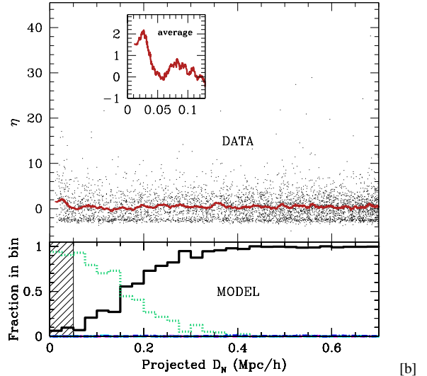
FIG. 8.— Star formation as a function of distance to nearest neighbor in sparse environments. (Top) For the 2dFGRS sample with N_{700} = 1 , we plot \eta as a function of separation to the nearest neighbor; the red line is the averaged smoothed by 100 points. The inset displays the average for D_N \lesssim 0.13 \text{ h}^{-1} \text{ Mpc} , highlighting the signal of triggered star formation at D_N \lesssim 0.03 \text{ h}^{-1} \text{ Mpc} . (Bottom) For the N_{700} = 1 sample in the simulation, we plot the fraction of N = 1 (solid, black) and N = 2 (dotted, green) galaxies as a function of D_N , as in Fig. 5.
