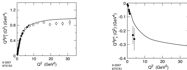
Fig. 7. Predictions for Q^4 F_1^p(Q^2) and Q^4 F_1^n(Q^2) in the soft wall model for \kappa = 0.424 GeV. The data compilation is from Diehl. 59
