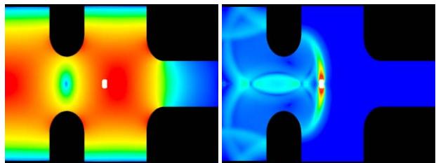
Figure 2: Cross-section of LCLS RF gun, showing electric field magnitude as calculated with Pic2P. (Left) Particle bunch accelerated by operating mode, (Right) scattered fields from interactions of bunch with gun cavity.
