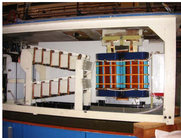
Figure 1: View of resonating capacitor, nanocrystalline boost transformer, and resonant rectification assembly
