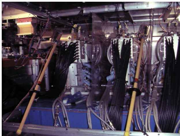
Figure 3: IGBT switching assemblies
